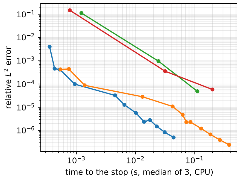
Bratu (error against the p = 48 reference)
