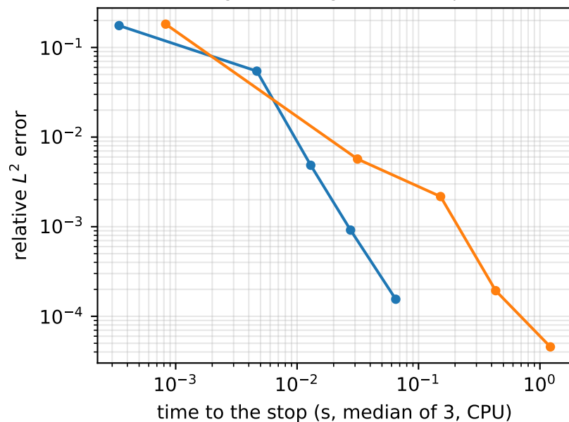
Burgers (error against Cole-Hopf)
