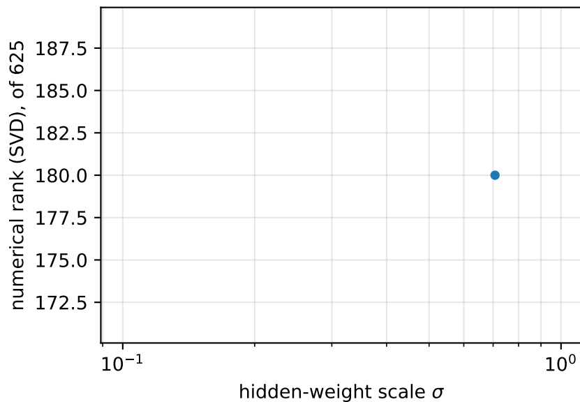
Burgers, P = 625 tanh random features: median over seeds 0-4, min-max band
