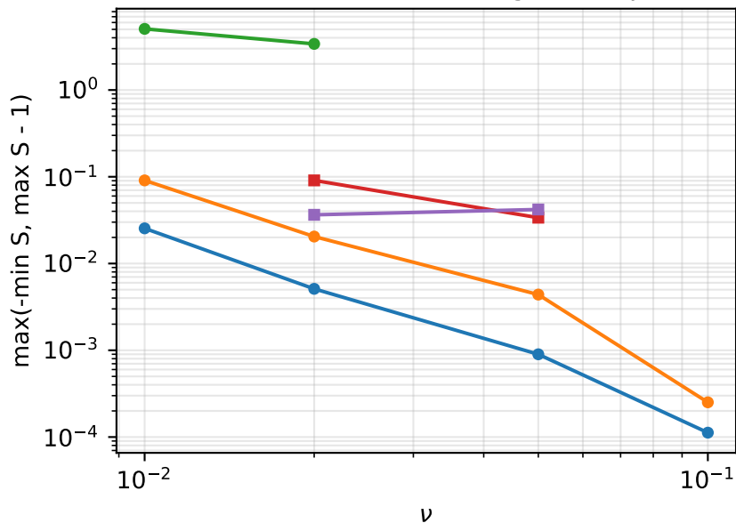
overshoot on the test grid (stop)
