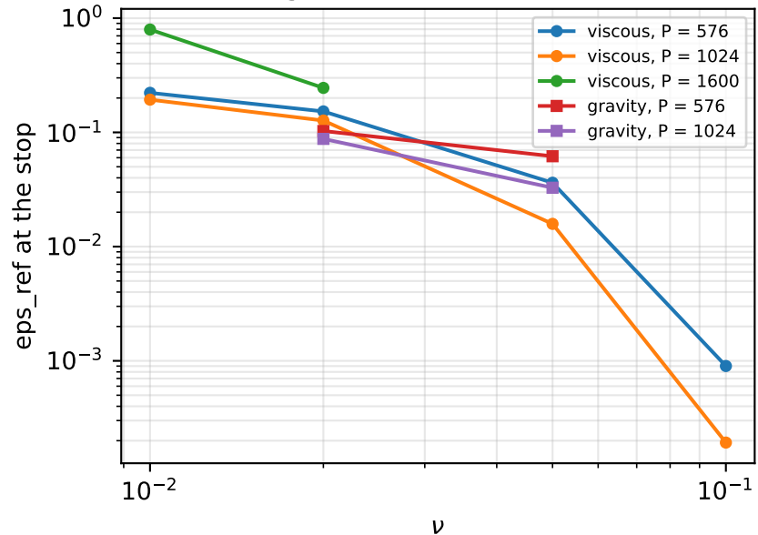
error against the refined reference
