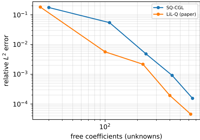
Burgers (error against Cole-Hopf)
