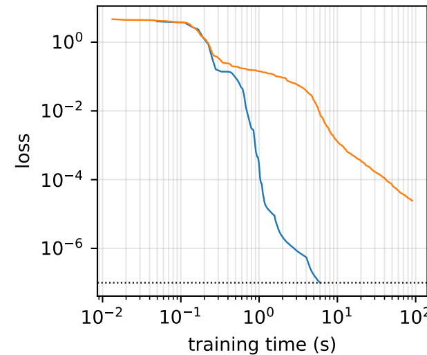
burgers, P = 400
