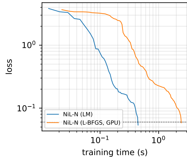
burgers, P = 25
