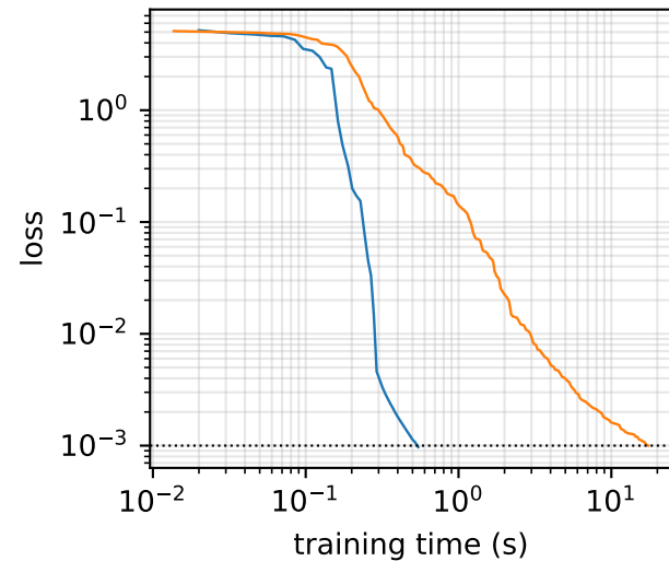
burgers, P = 100
