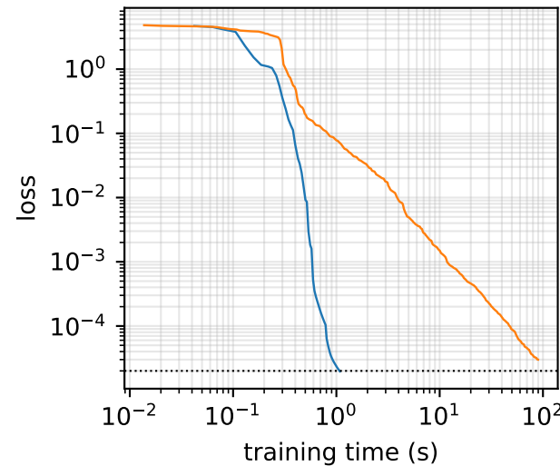
burgers, P = 225
