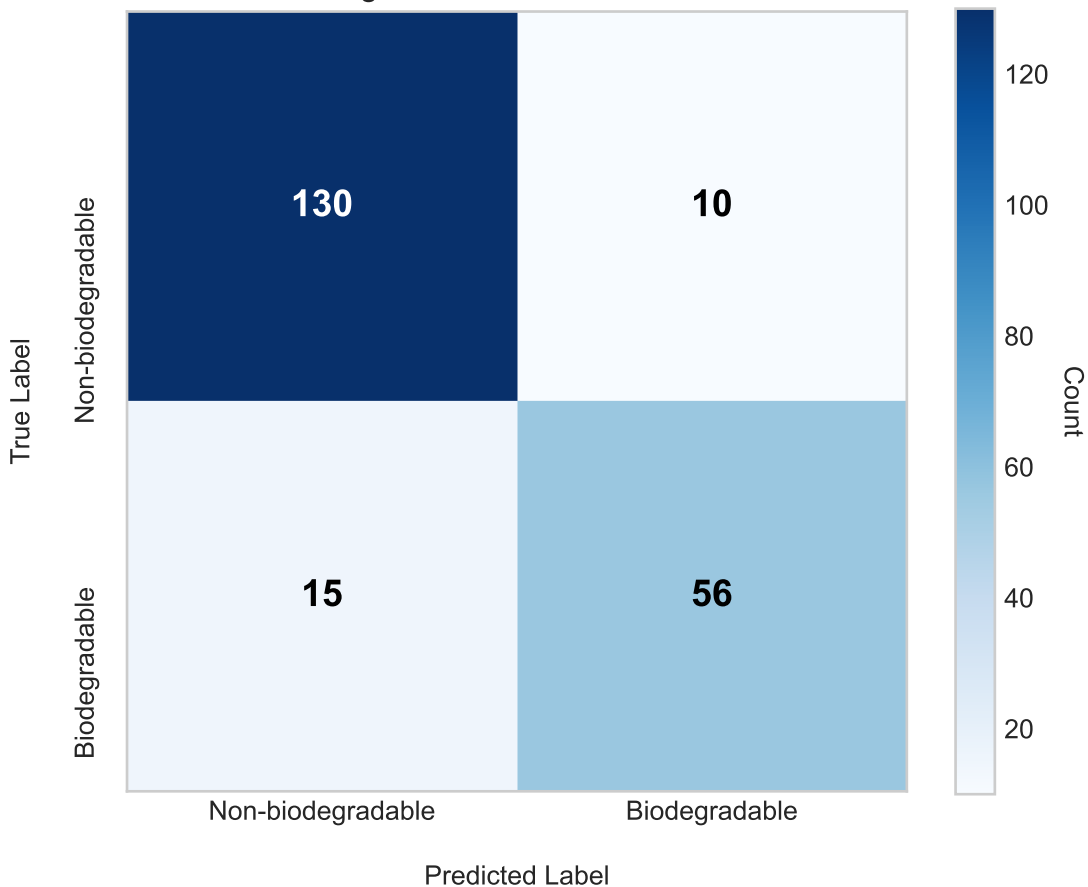
Stacking Ensemble Confusion Matrix
