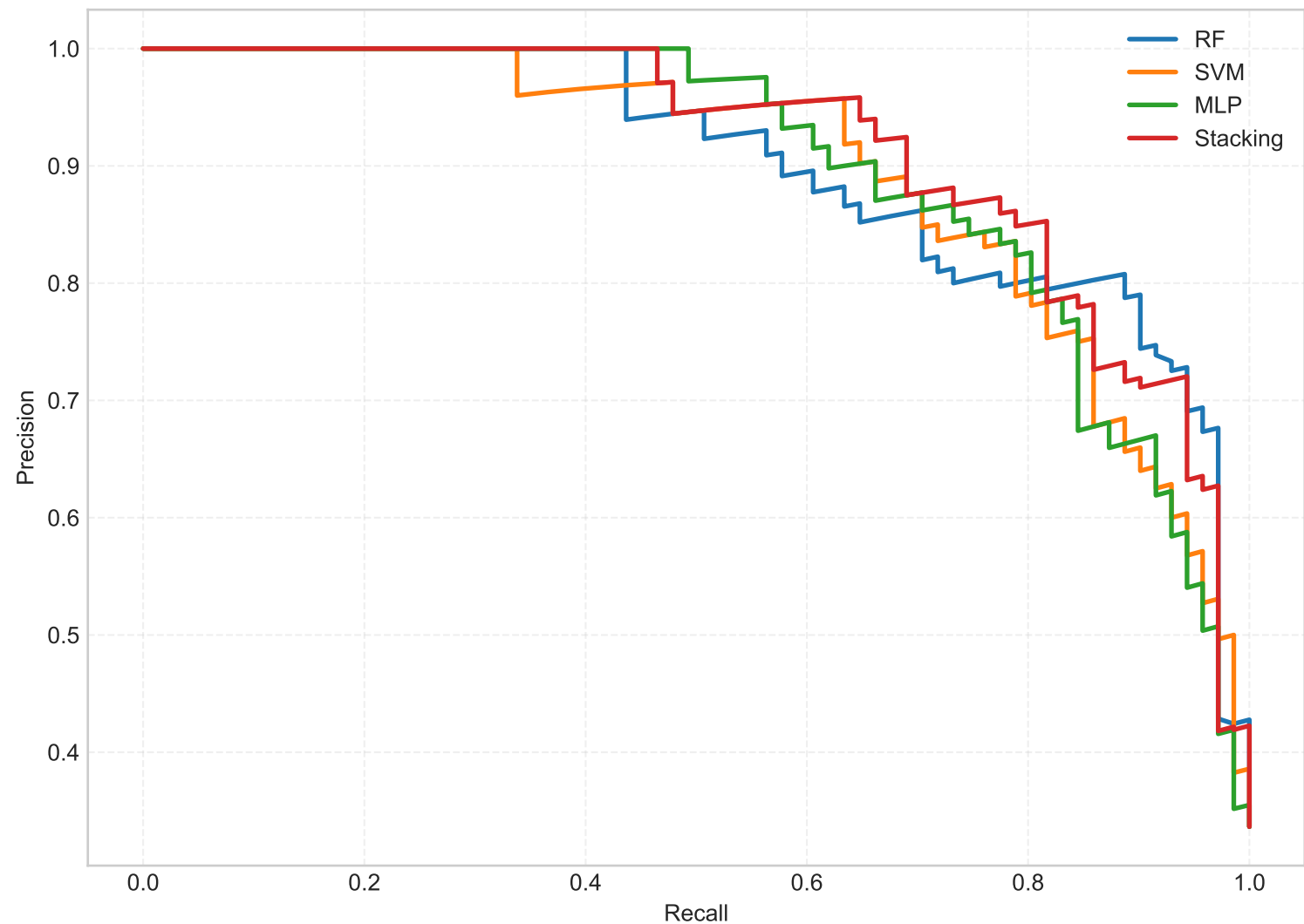
Precision-Recall Curves
