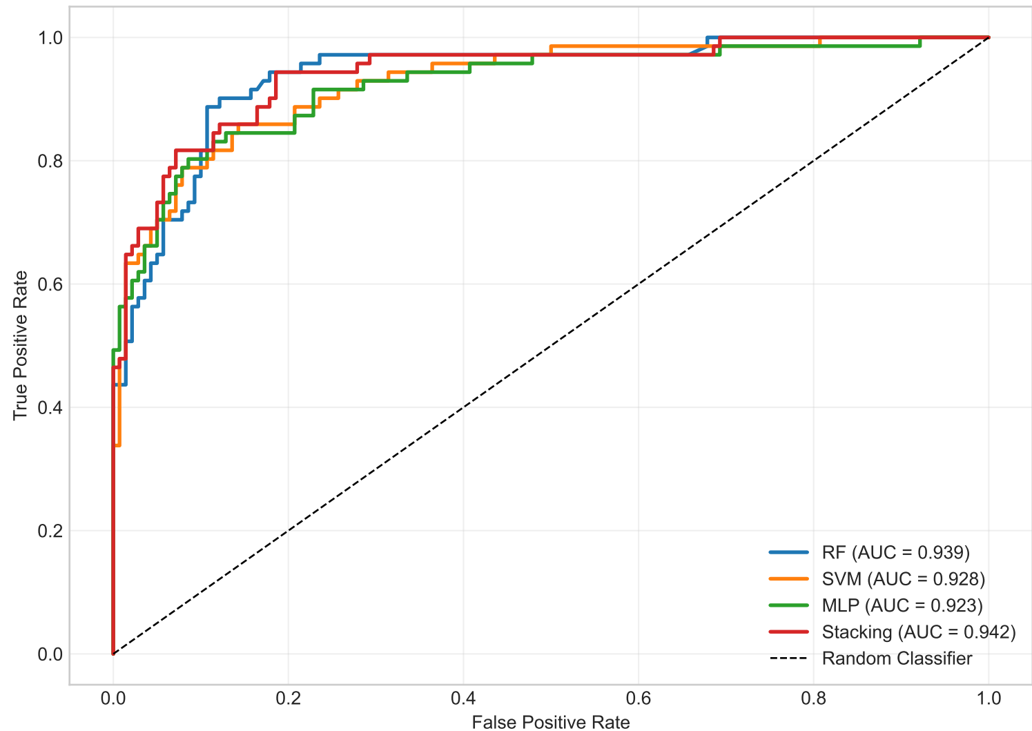
ROC Curves: Classifier Comparison
