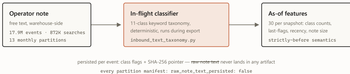
FIGURE 6 The inbound text layer. Signal crosses the boundary; text does not. The one taxonomy class that never fired ( undeliverable : 60 hits in 17.9M events) shipped as a dead feature and is first in line for the v2 phrasing pass.
