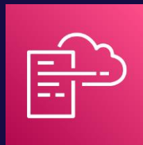
AWS CloudFormation
