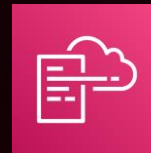
CloudFormation hooks
