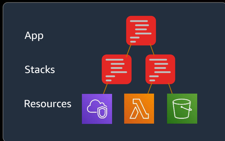
Core framework
