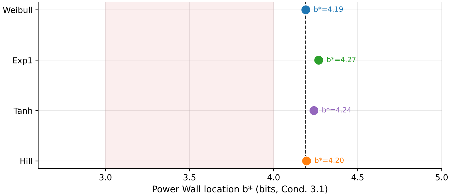
Fig 19. Model-Form Robustness — b^* across alternative functional forms
