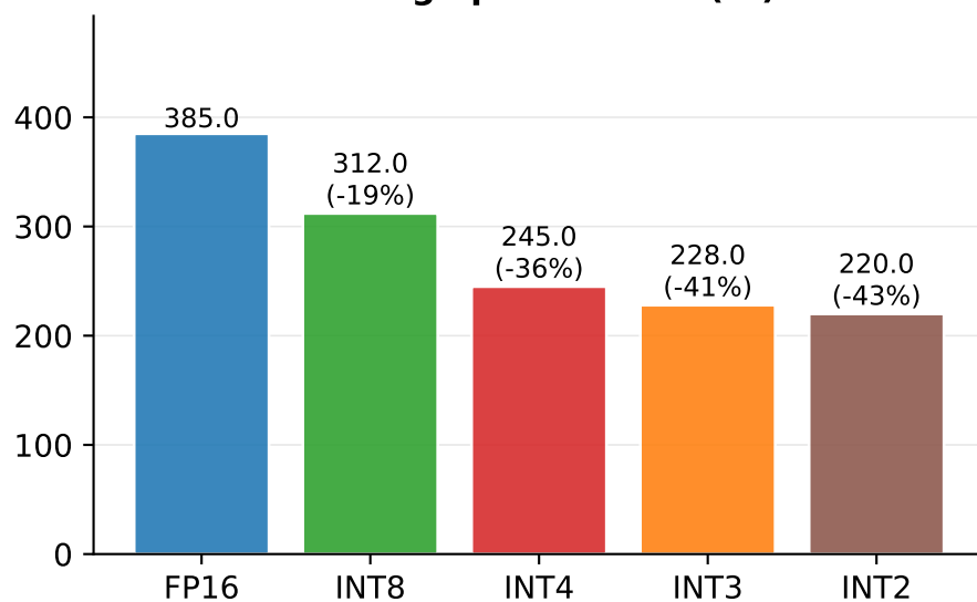
Throughput (tokens/s)
