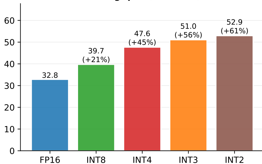
Throughput (tokens/s)
