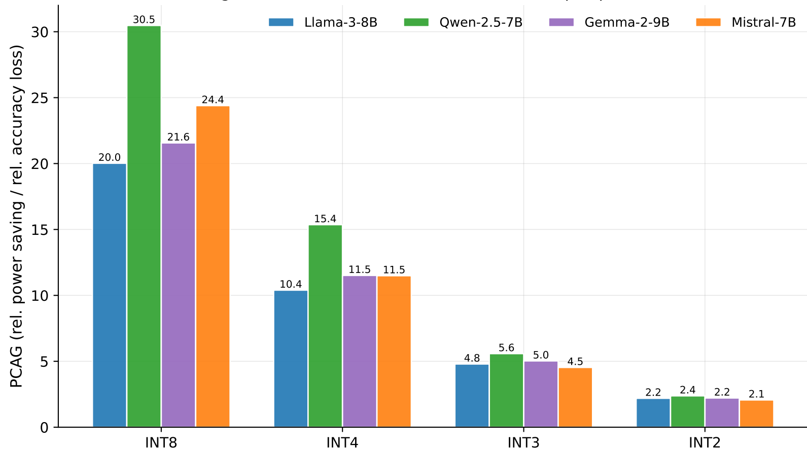
Fig 7. PCAG across Models — universal collapse pattern
