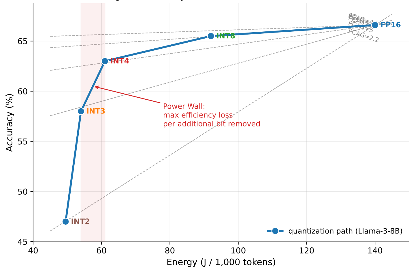
Fig 14. Efficiency Frontier with iso-PCAG contours
