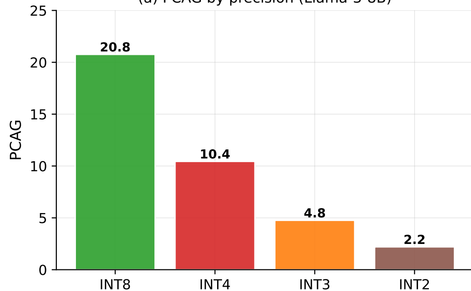
(a) PCAG by precision (Llama-3-8B)
