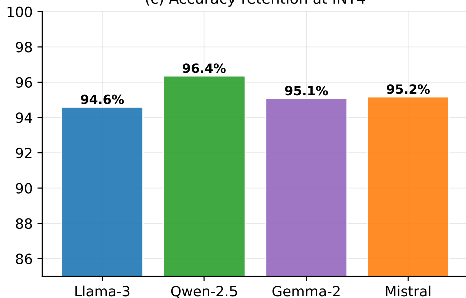
(c) Accuracy retention at INT4
