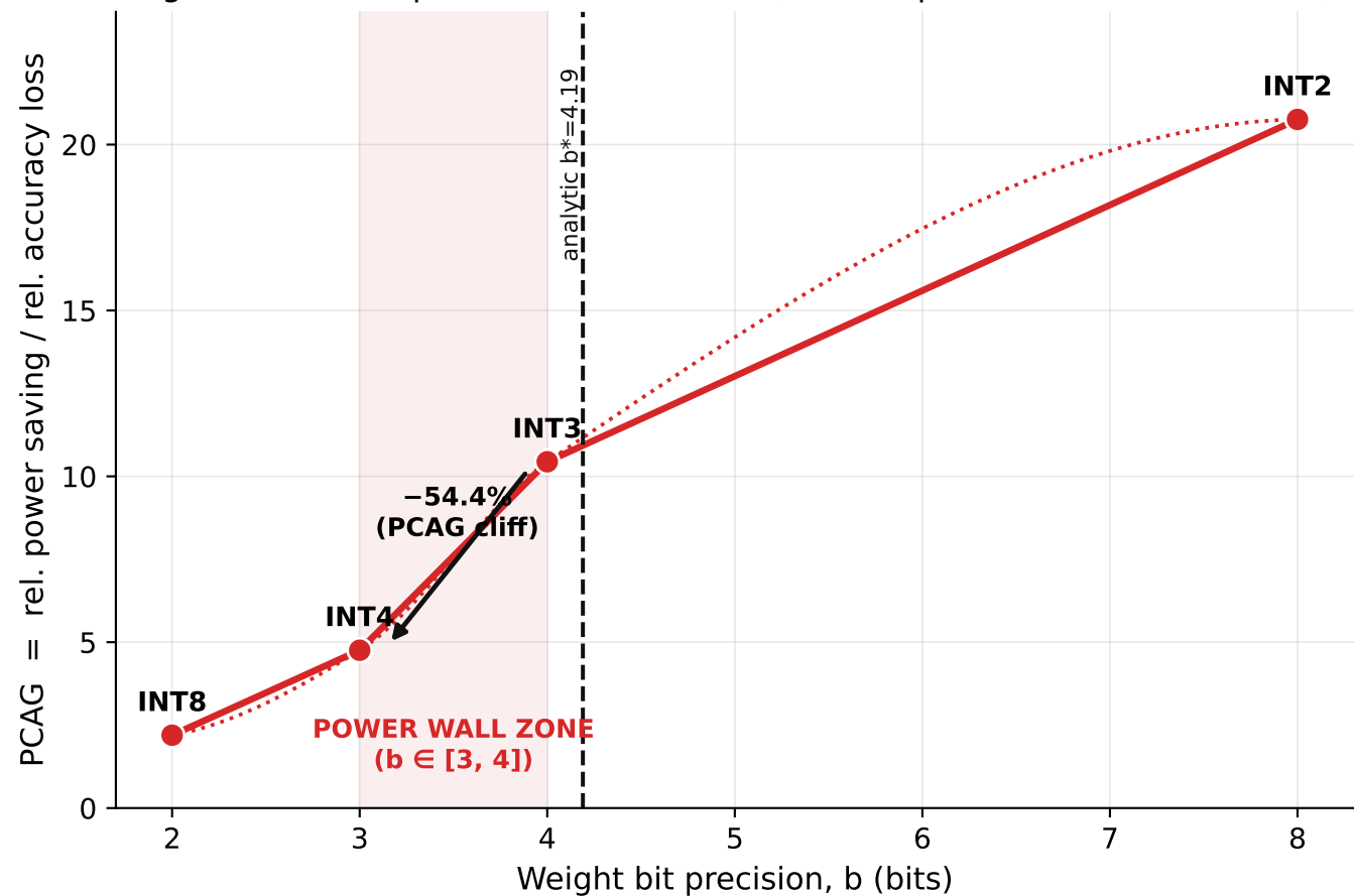
Fig 2. PCAG Collapse — the Power Wall ( \theta=3 , slope 5.68/bit at INT4 \rightarrow INT3)
