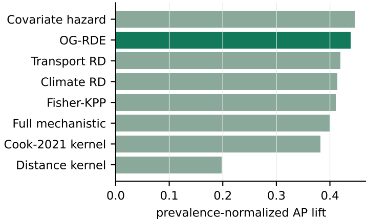
Skill beyond frozen-target prevalence
