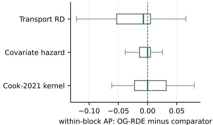
Where does OG-RDE add value?
