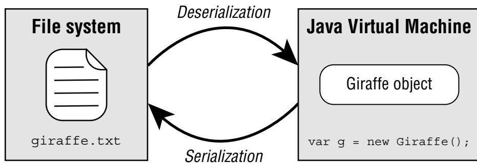
FIGURE 14.6 Serialization process
