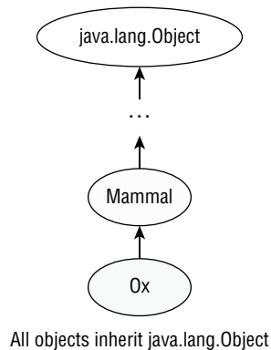
FIGURE 6.3 Java object inheritance
