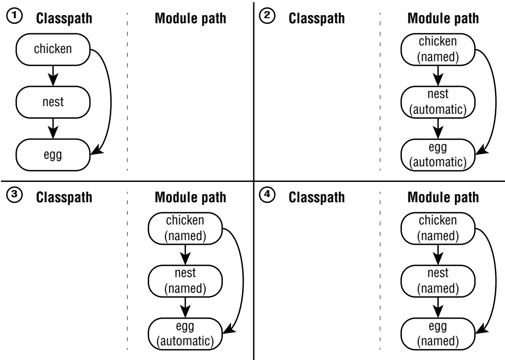
FIGURE 12.17 Top-down migration
