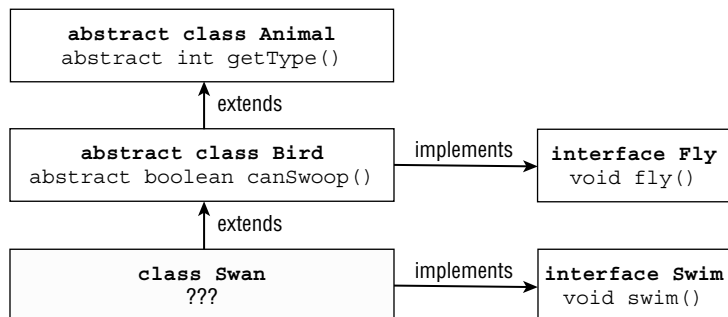
FIGURE 7.3 Interface Inheritance
