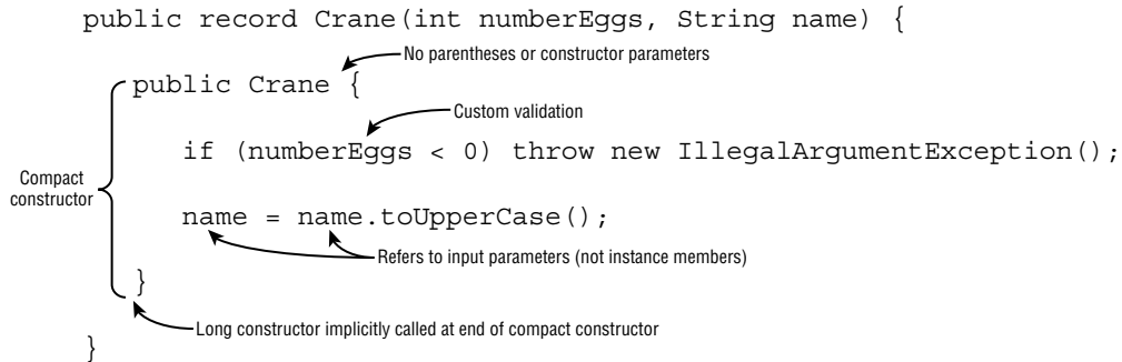
FIGURE 7.7 Declaring a compact constructor
