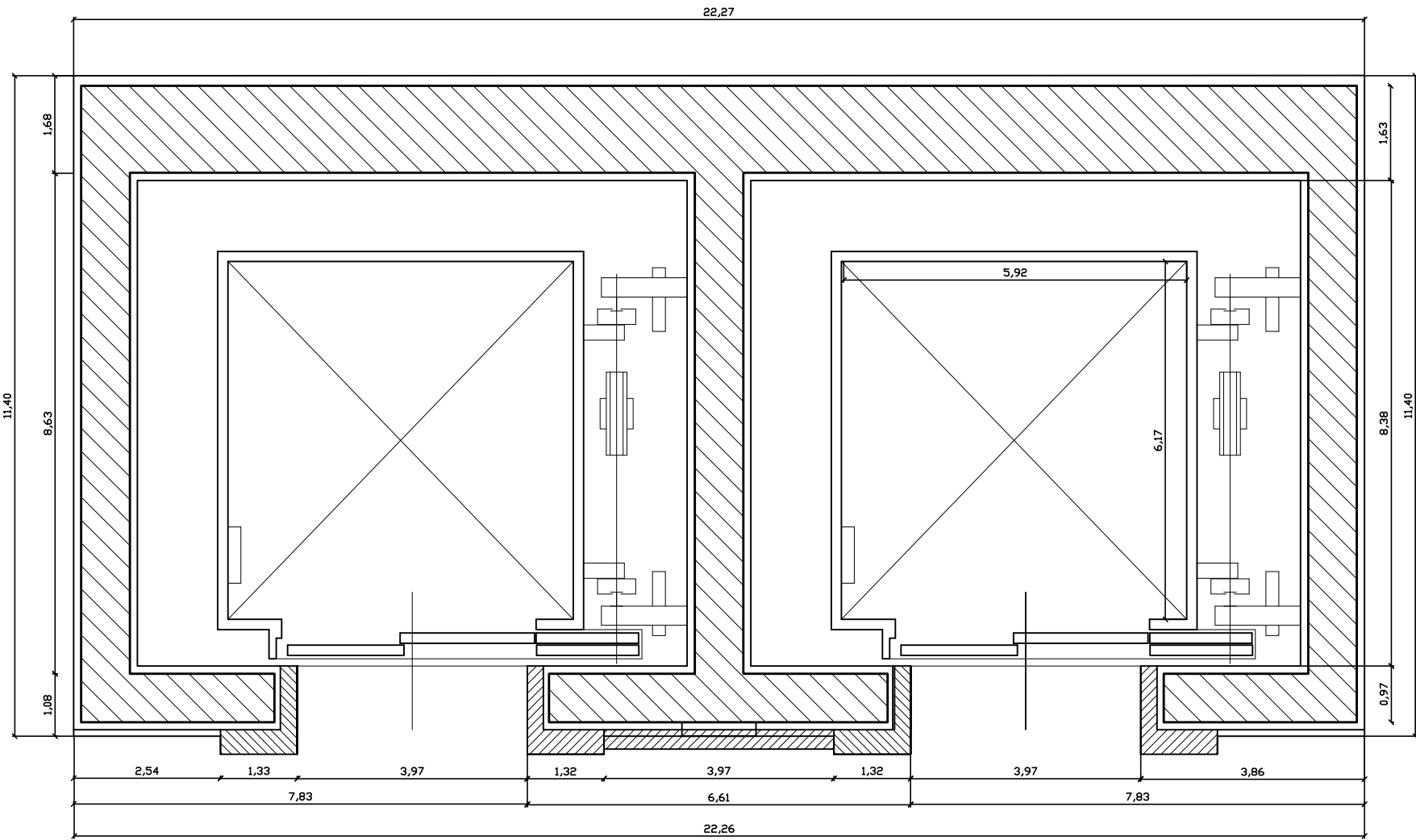
elevator plan 1:20
