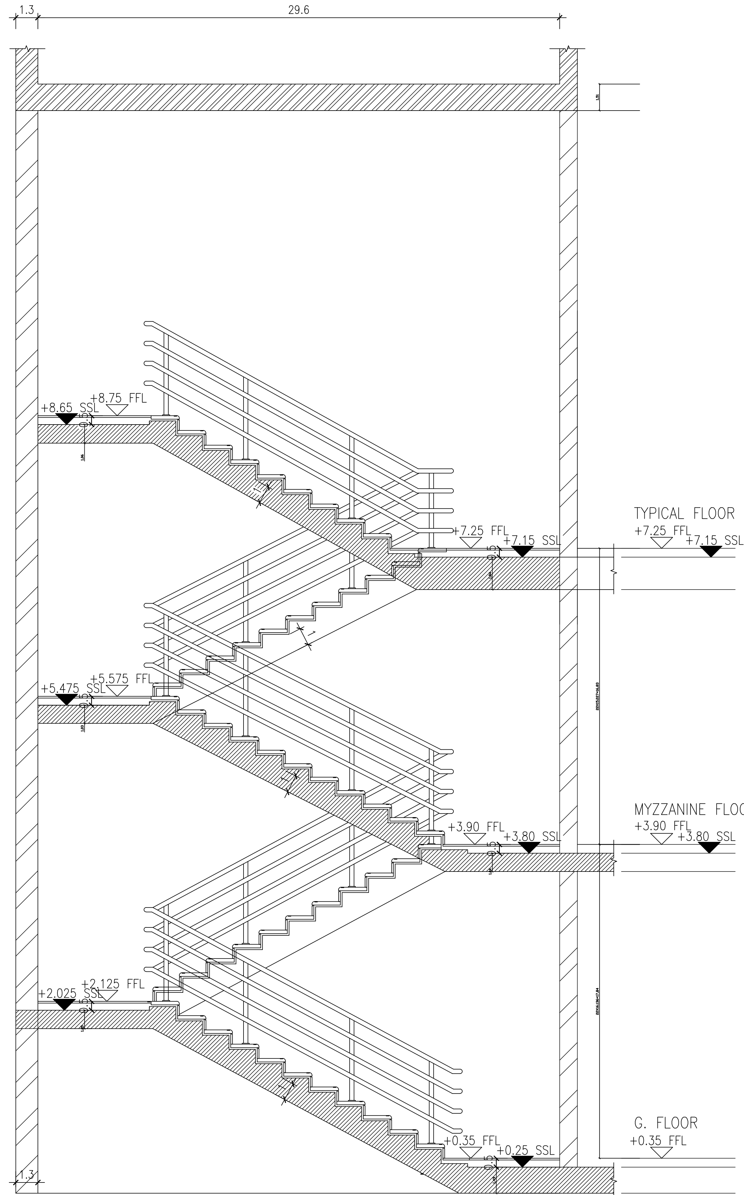
Stairs section 1:20
