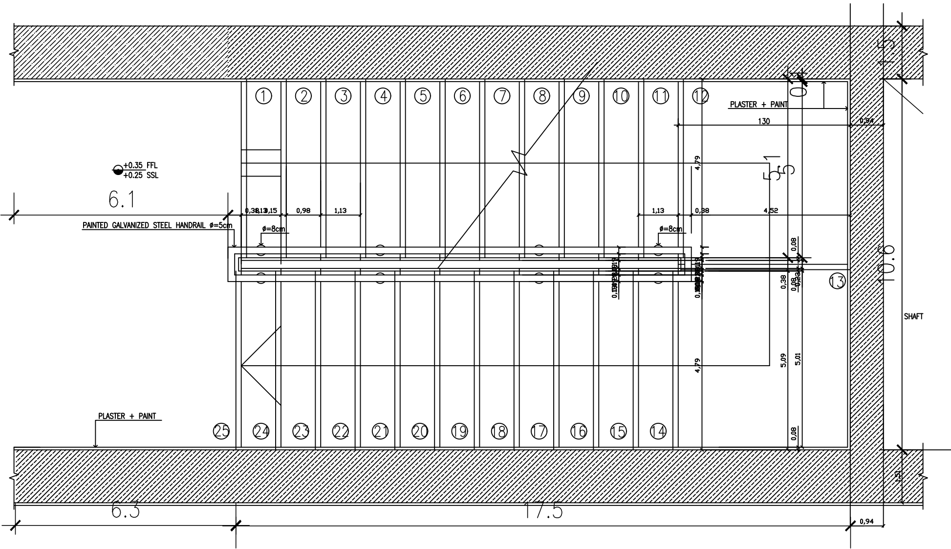
Stairs plan 1:20
