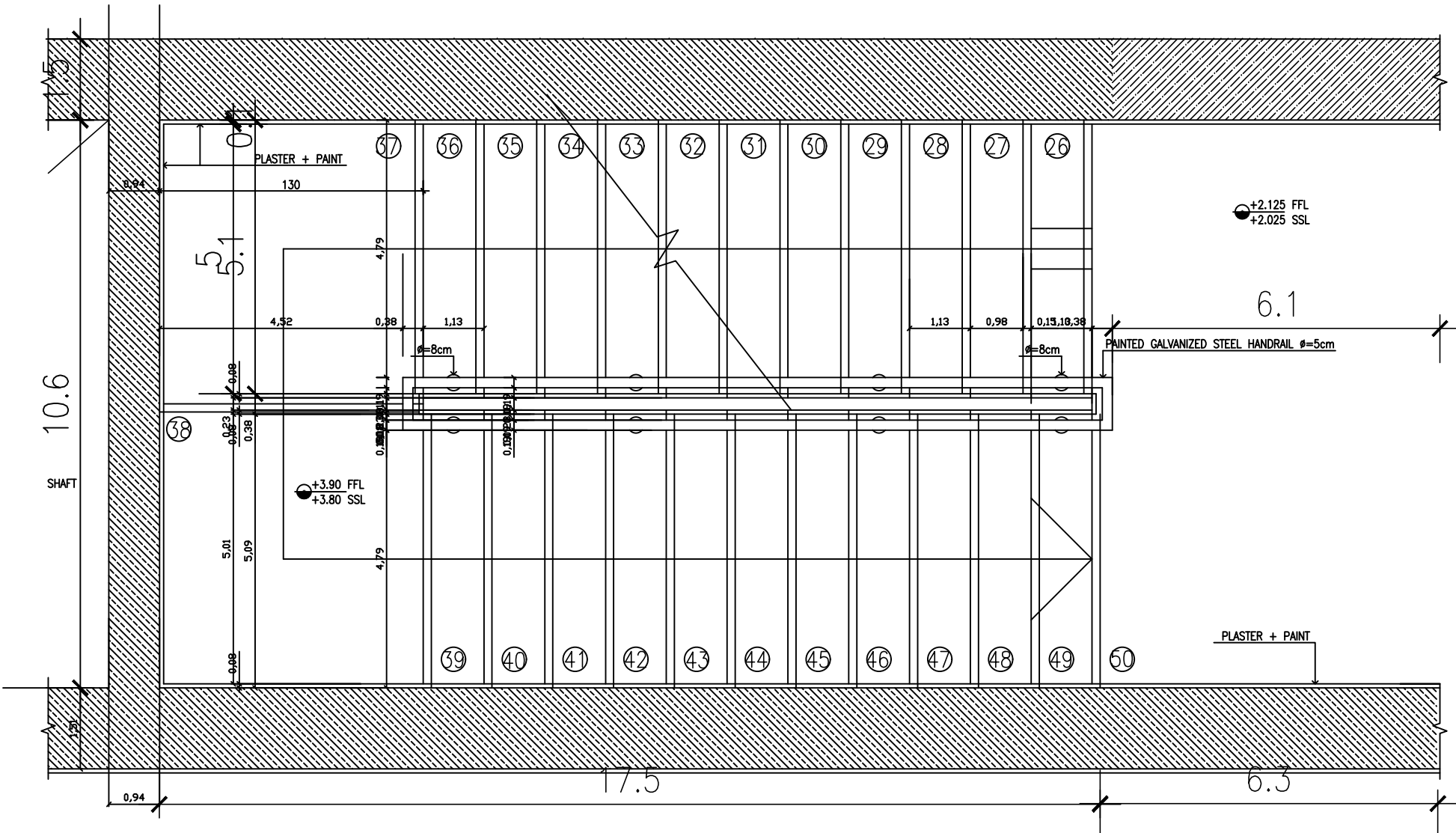
Stairs plan 1:20
