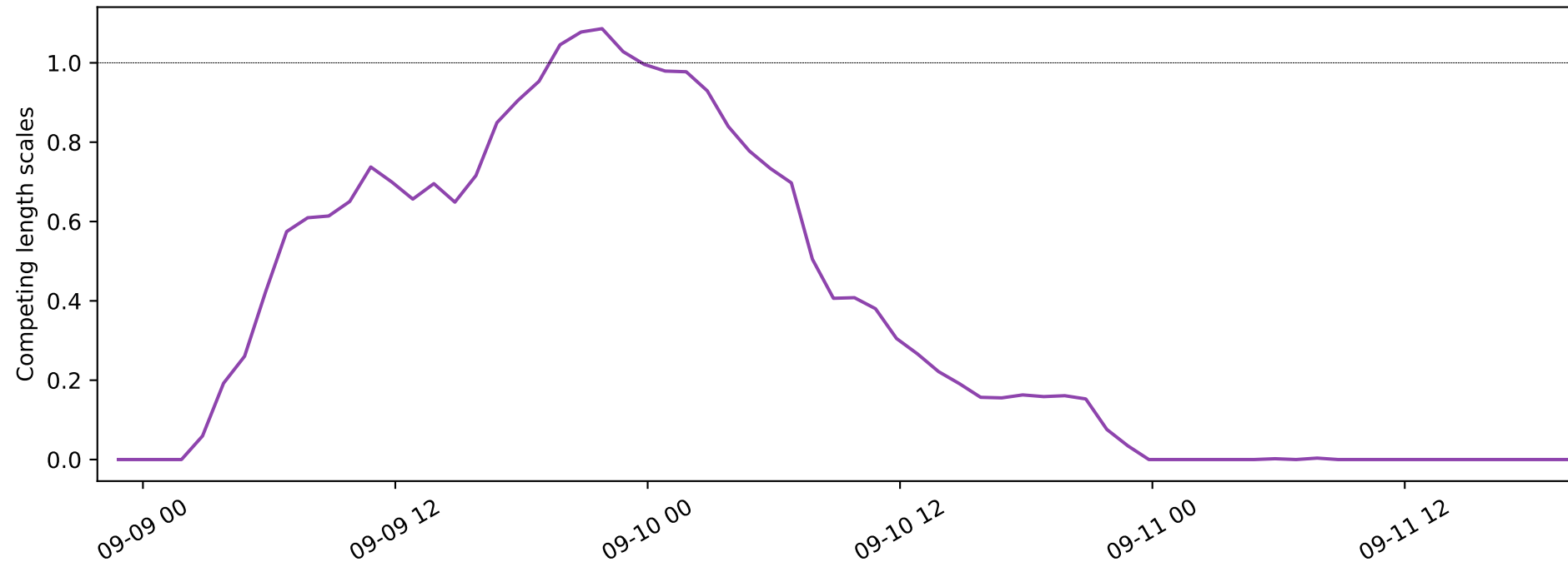
Distance to Qhull / sqrt(Qhull area), skill score: 0.65
