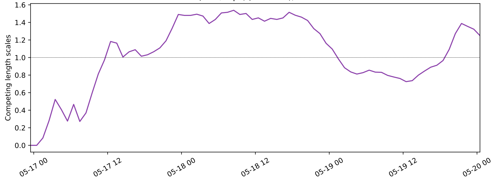
Distance to Qhull / sqrt(Qhull area), skill score: -0.04
