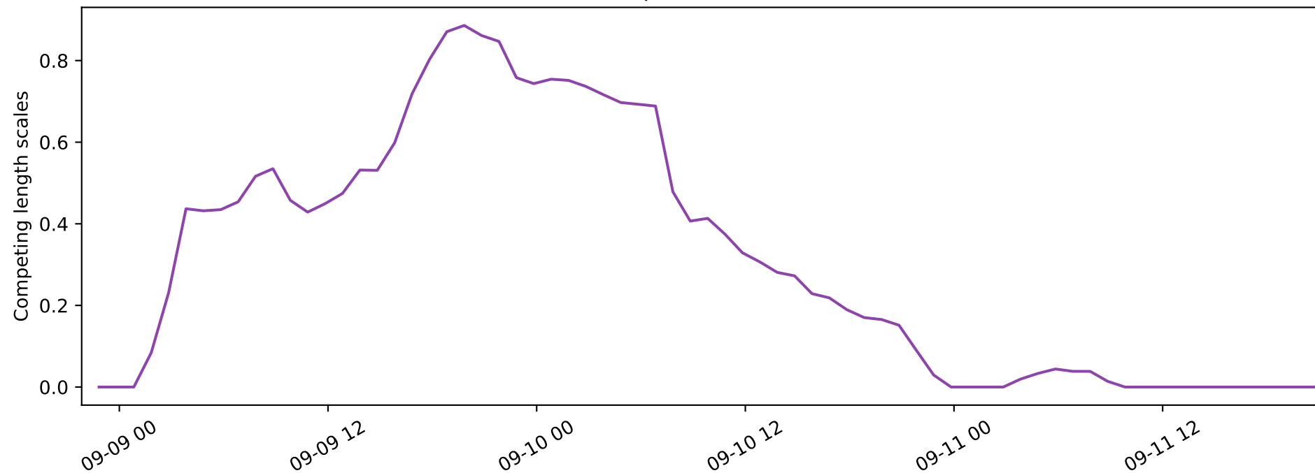
Distance to Qhull / sqrt(Qhull area), skill score: 0.69
