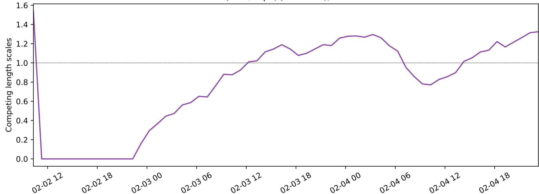
Distance to Qhull / sqrt(Qhull area), skill score: 0.21
