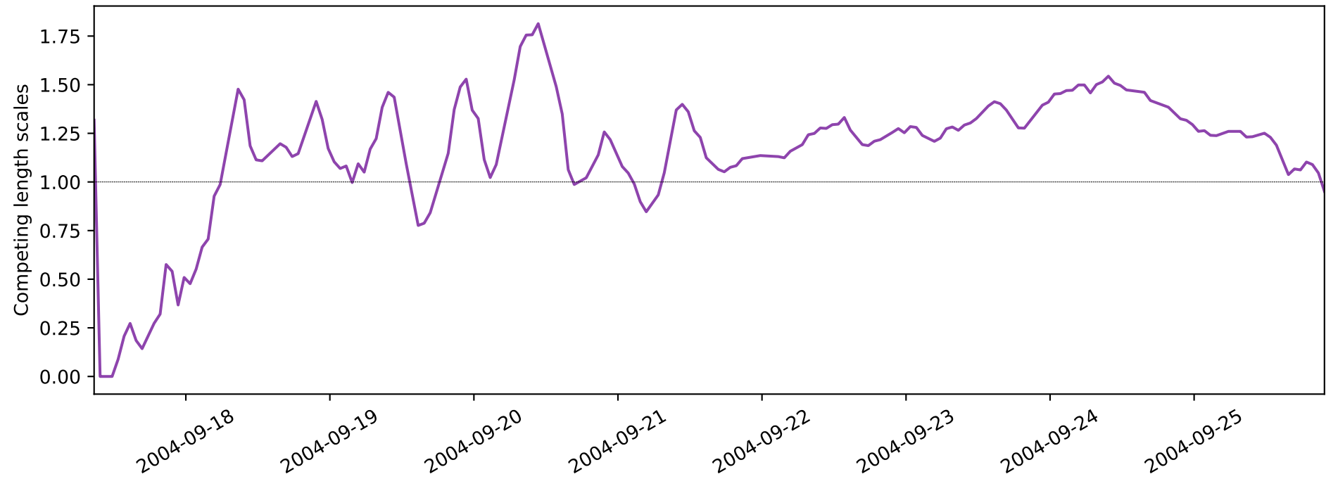
Distance to Qhull / sqrt(Qhull area), skill score: -0.16
