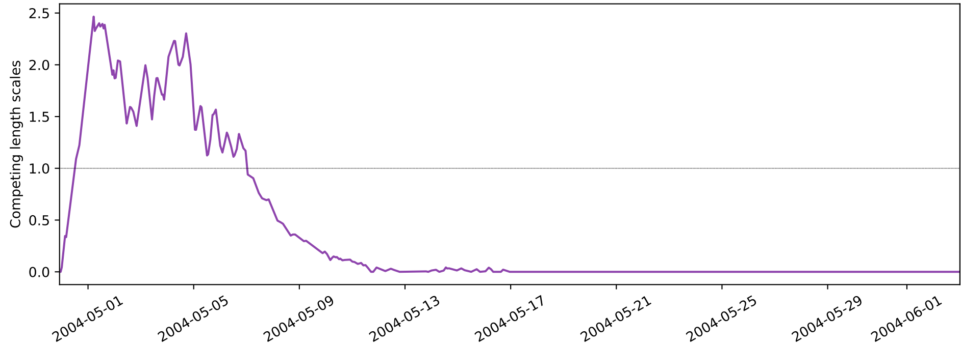
Distance to Qhull / sqrt(Qhull area), skill score: 0.62
