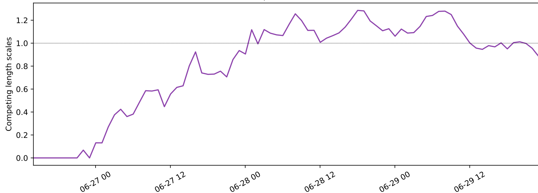
Distance to Qhull / sqrt(Qhull area), skill score: 0.19
