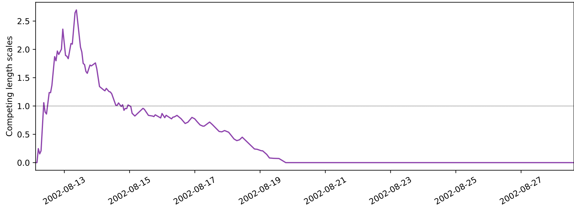
Distance to Qhull / sqrt(Qhull area), skill score: 0.58
