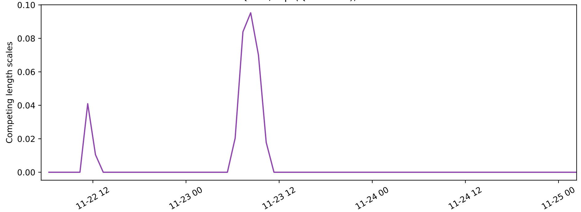
Distance to Qhull / sqrt(Qhull area), skill score: 1.00
