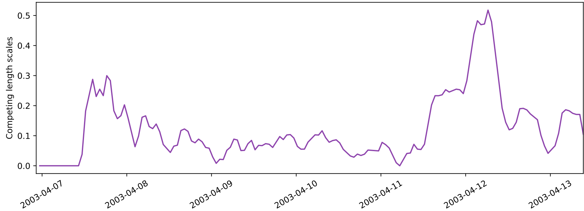
Distance to Qhull / sqrt(Qhull area), skill score: 0.88
