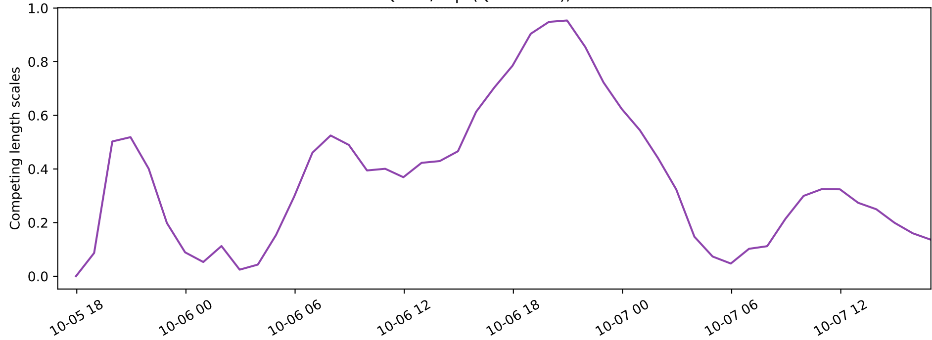
Distance to Qhull / sqrt(Qhull area), skill score: 0.64
