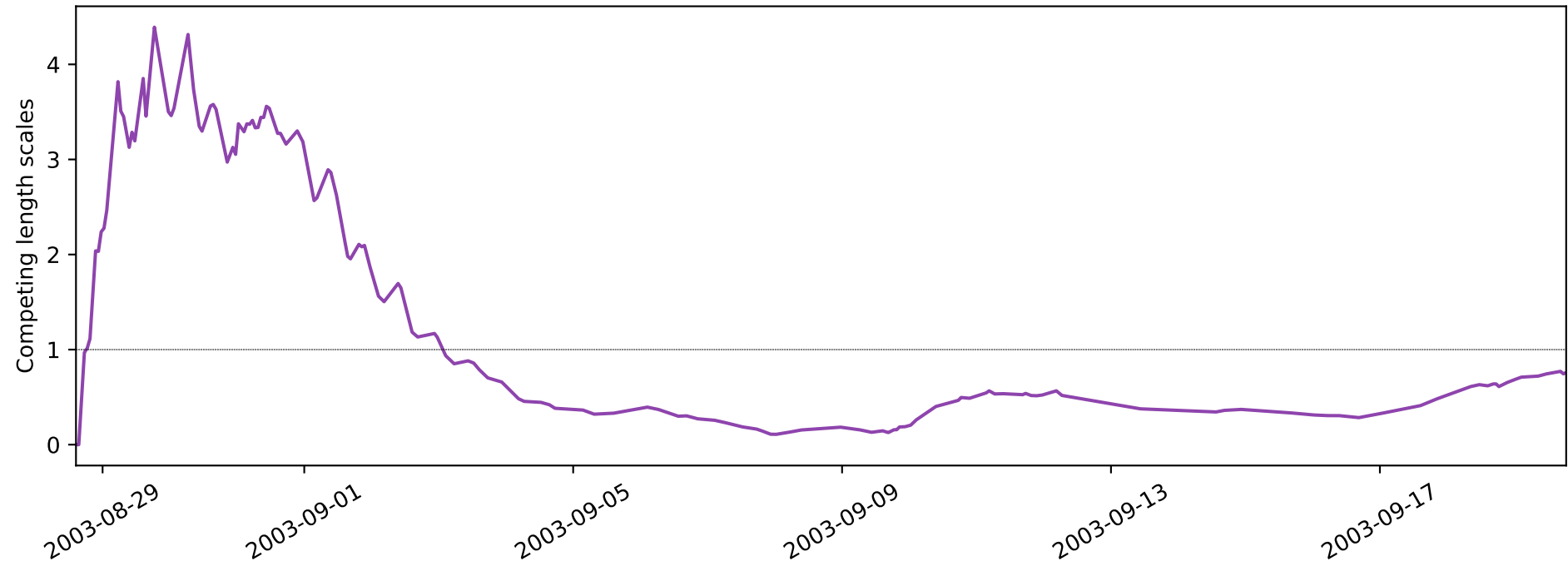
Distance to Qhull / sqrt(Qhull area), skill score: 0.03
