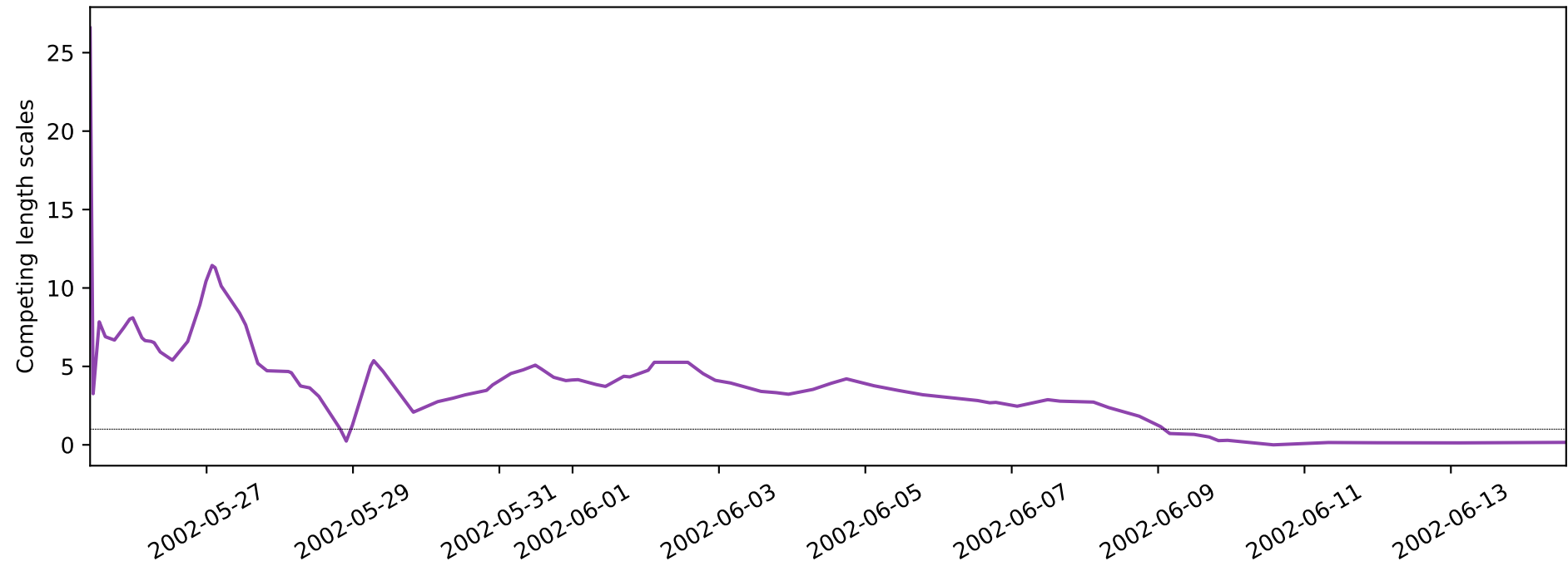
Distance to Qhull / sqrt(Qhull area), skill score: -2.08
