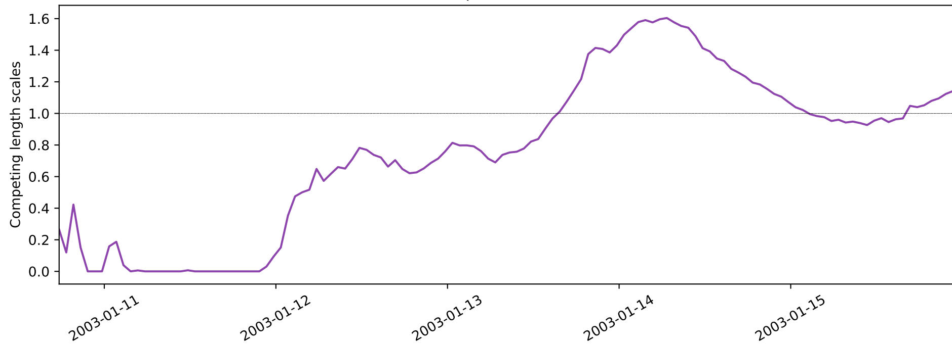
Distance to Qhull / sqrt(Qhull area), skill score: 0.24
