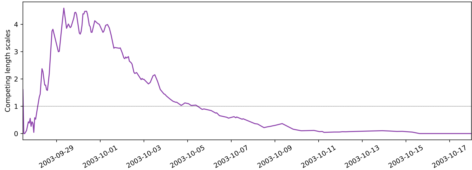
Distance to Qhull / sqrt(Qhull area), skill score: -0.09
