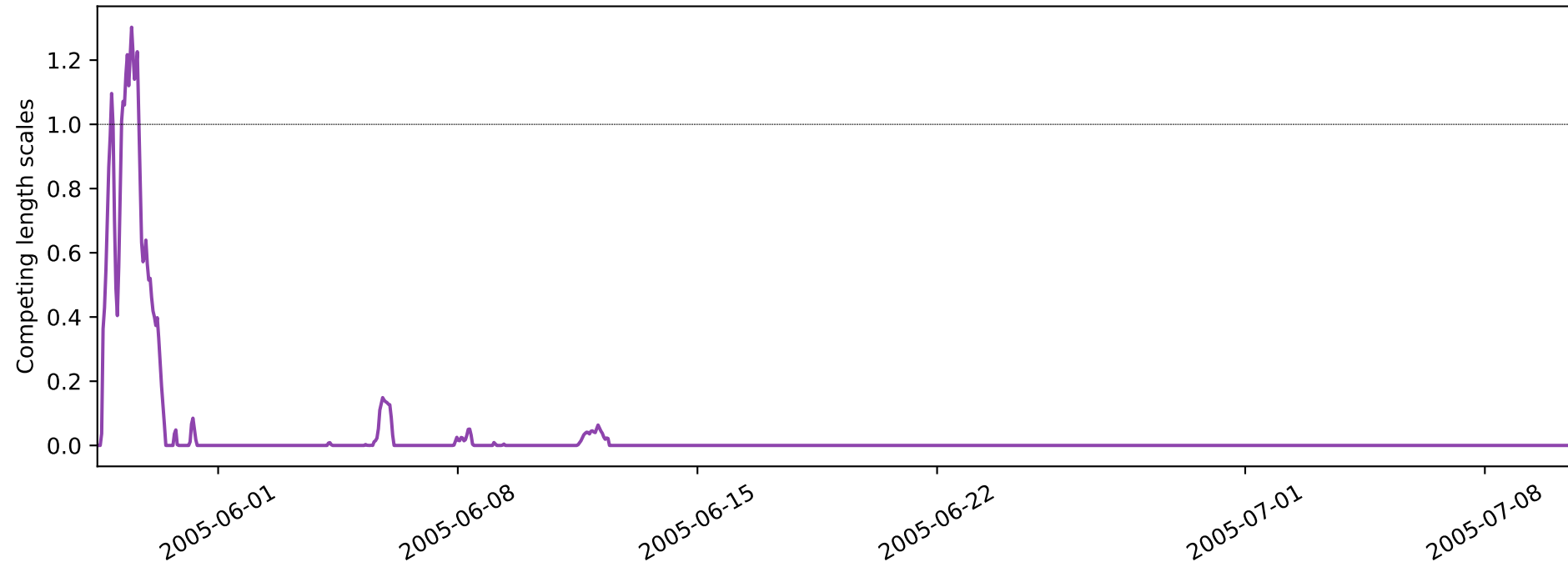
Distance to Qhull / sqrt(Qhull area), skill score: 0.97
