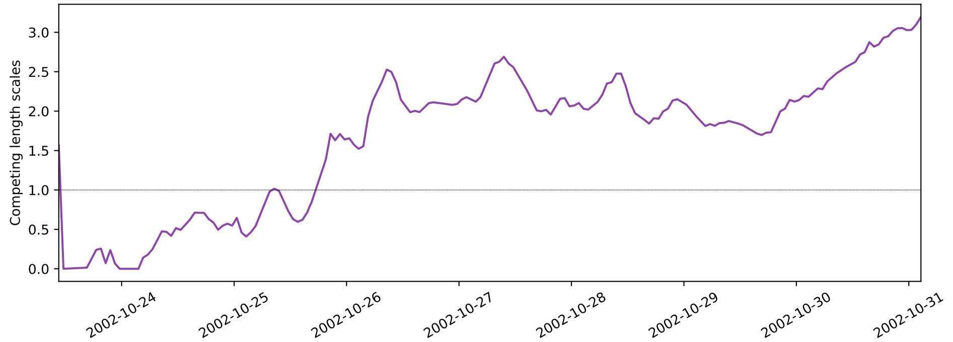
Distance to Qhull / sqrt(Qhull area), skill score: -0.66
