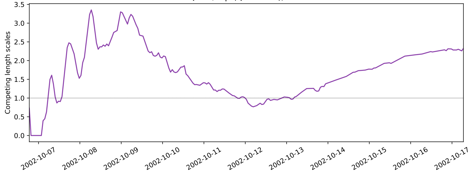
Distance to Qhull / sqrt(Qhull area), skill score: -0.71
