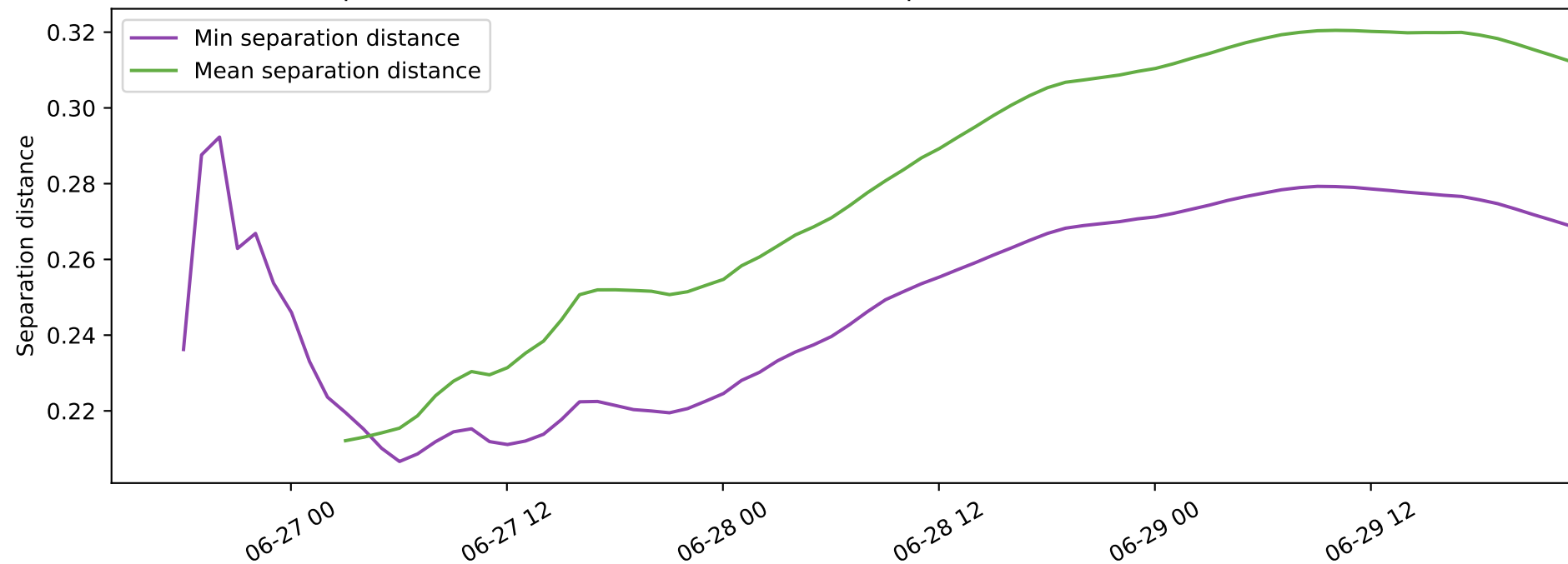
Separation distance, skill score: Max (min sep dist): 0.75, Mean: 0.57, Std: 0.91
