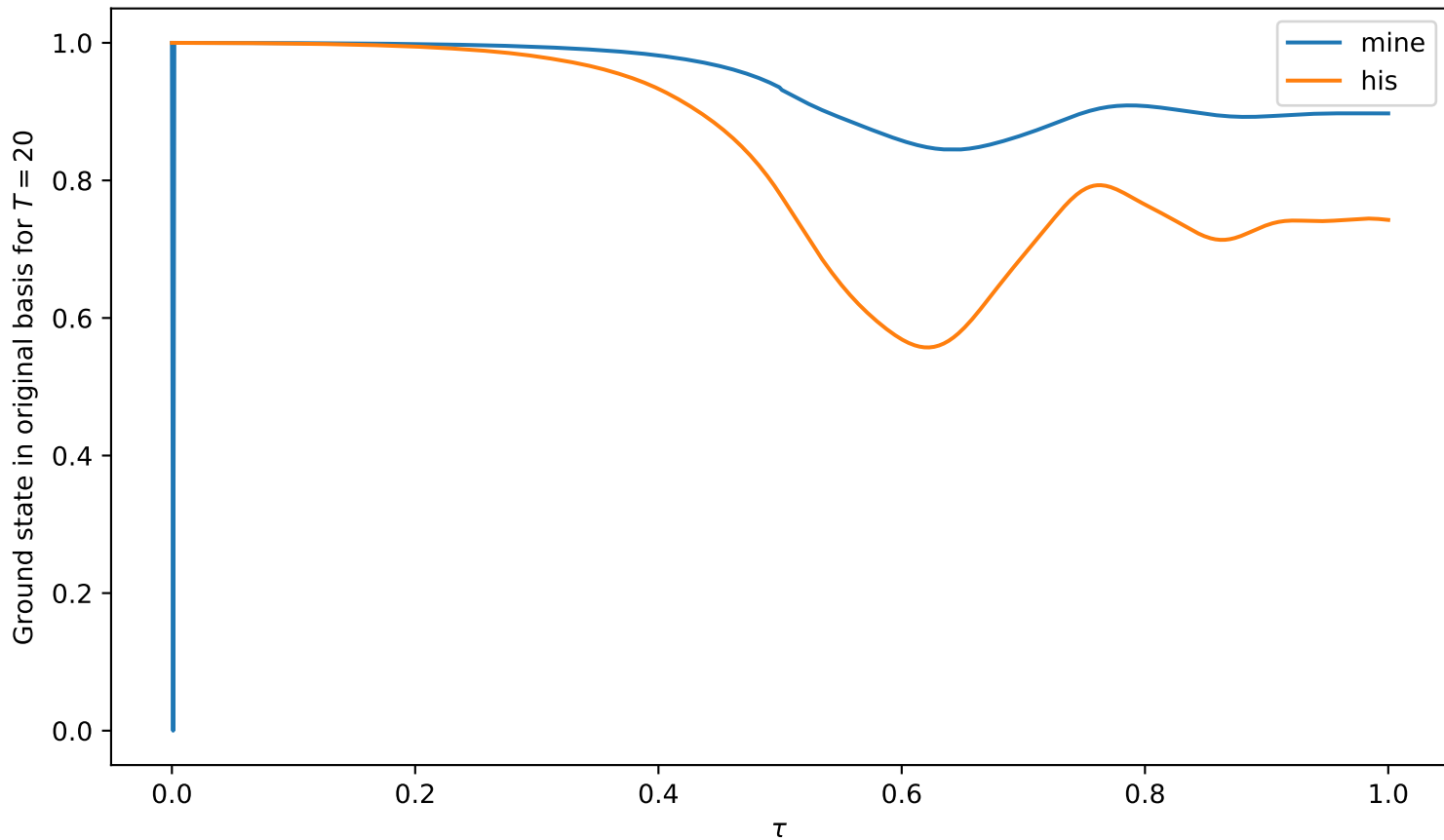
Ground-state coefficient comparison
