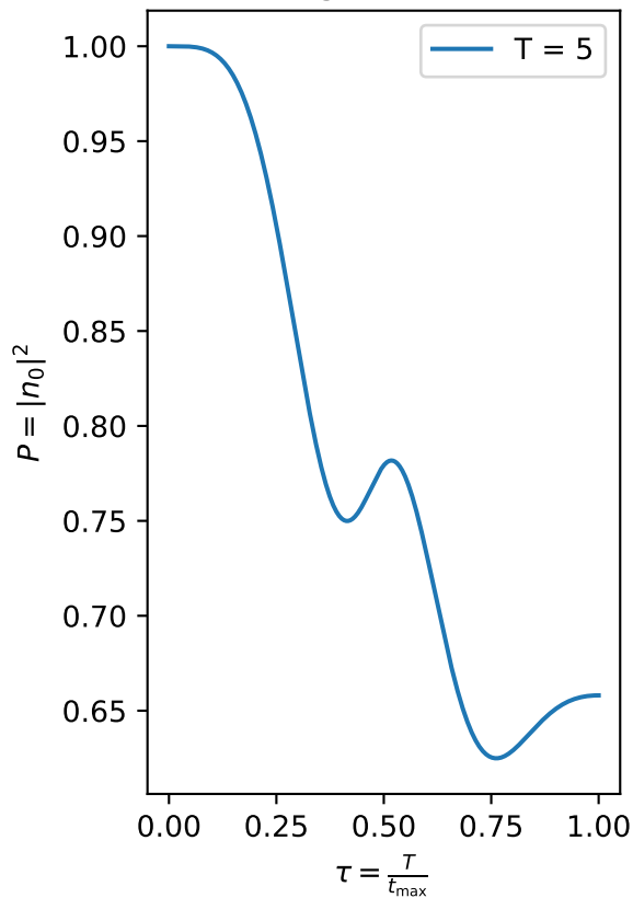
Original basis
