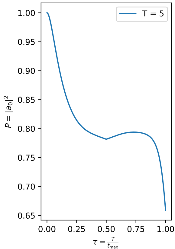
Adiabatic basis
