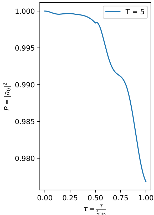
Adiabatic basis
