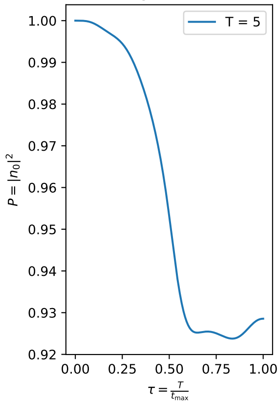
Original basis
