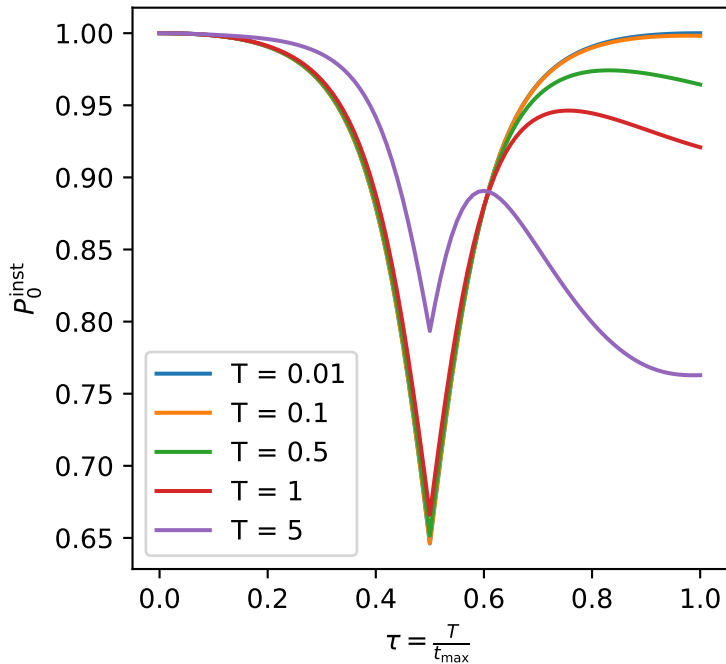
Instantan basis (Schrödinger)
