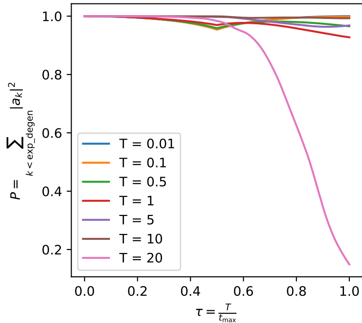
Instantan basis (Schrödinger)
