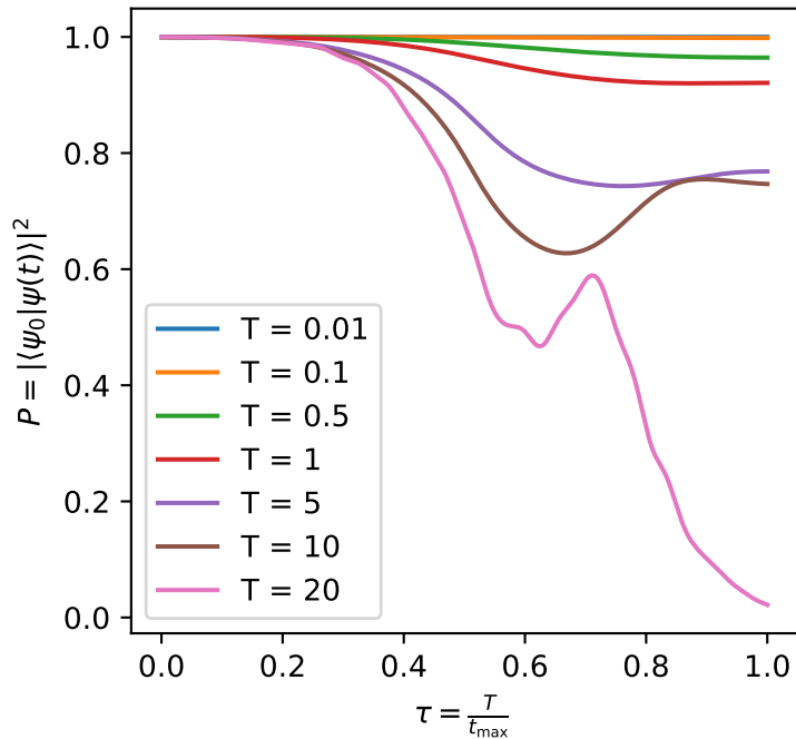
Original basis (Schrödinger)
