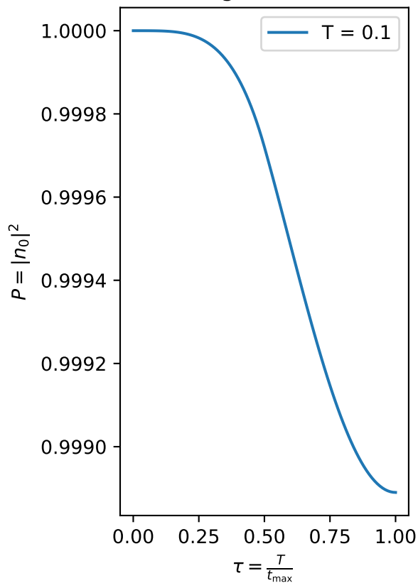
Original basis
