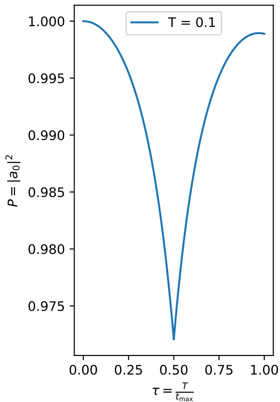
Adiabatic basis
