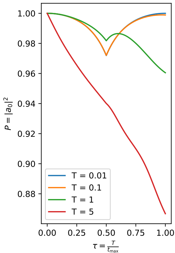
Adiabatic basis
