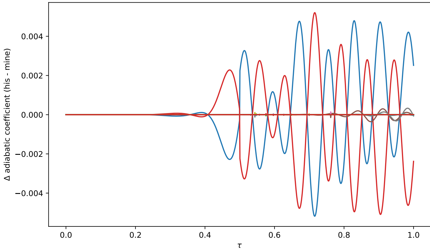
Difference in adiabatic basis coefficients at T_{\max} = 20
