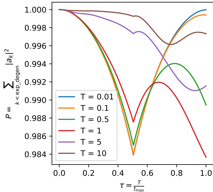
Instantan basis (Schrödinger)
