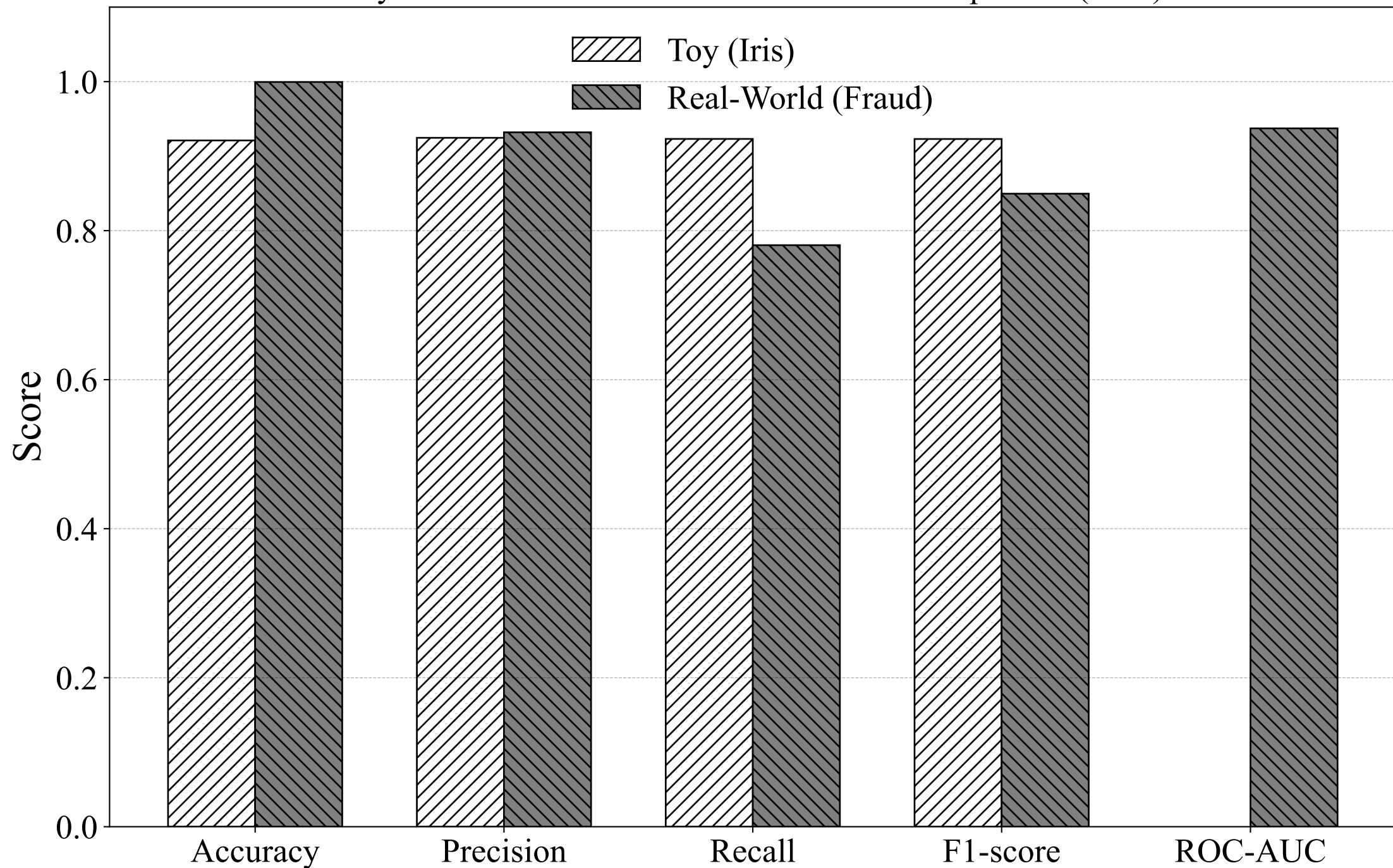
Toy vs. Real-World Dataset Performance Comparison (B/W)
