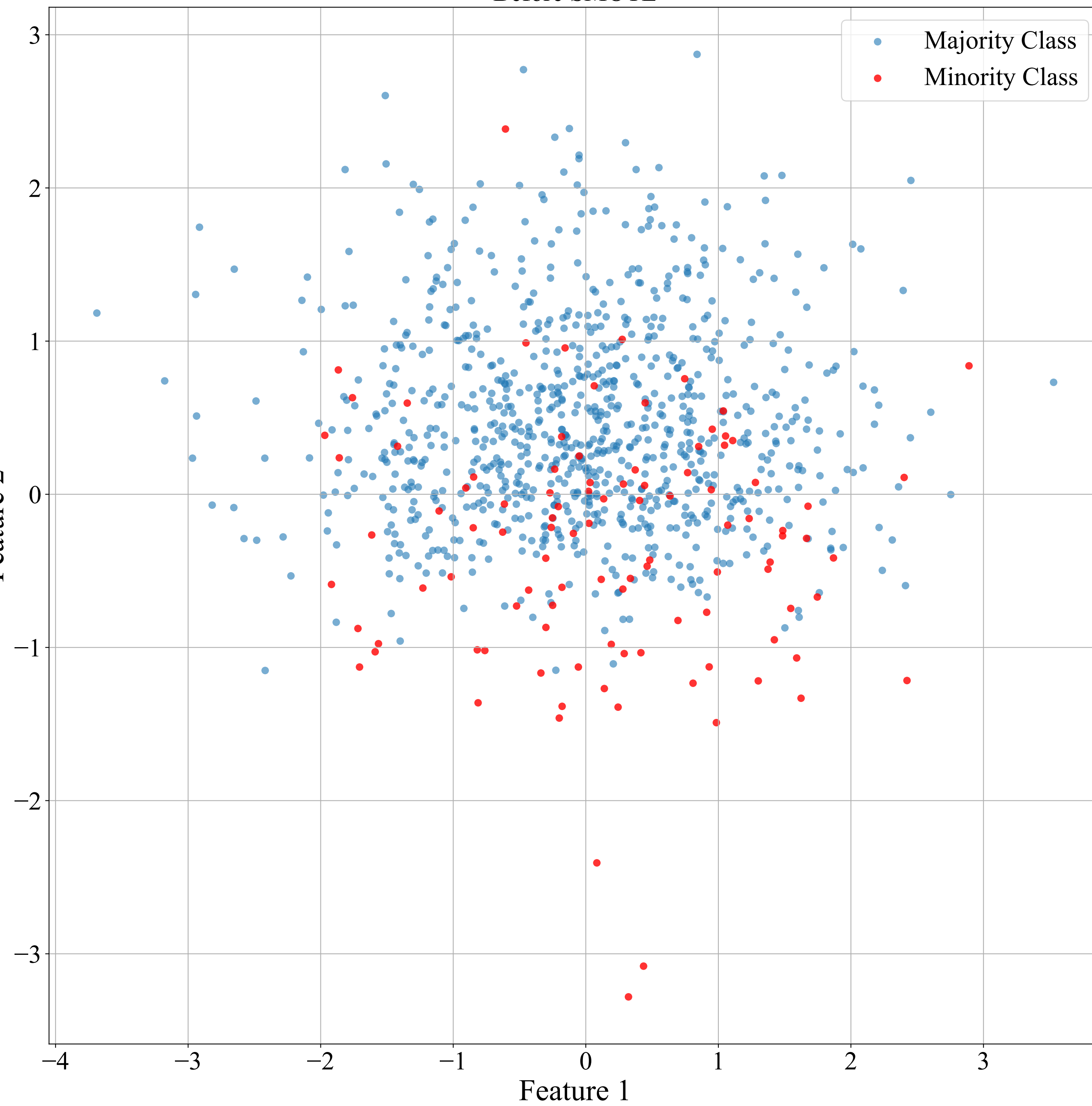
Before SMOTE
