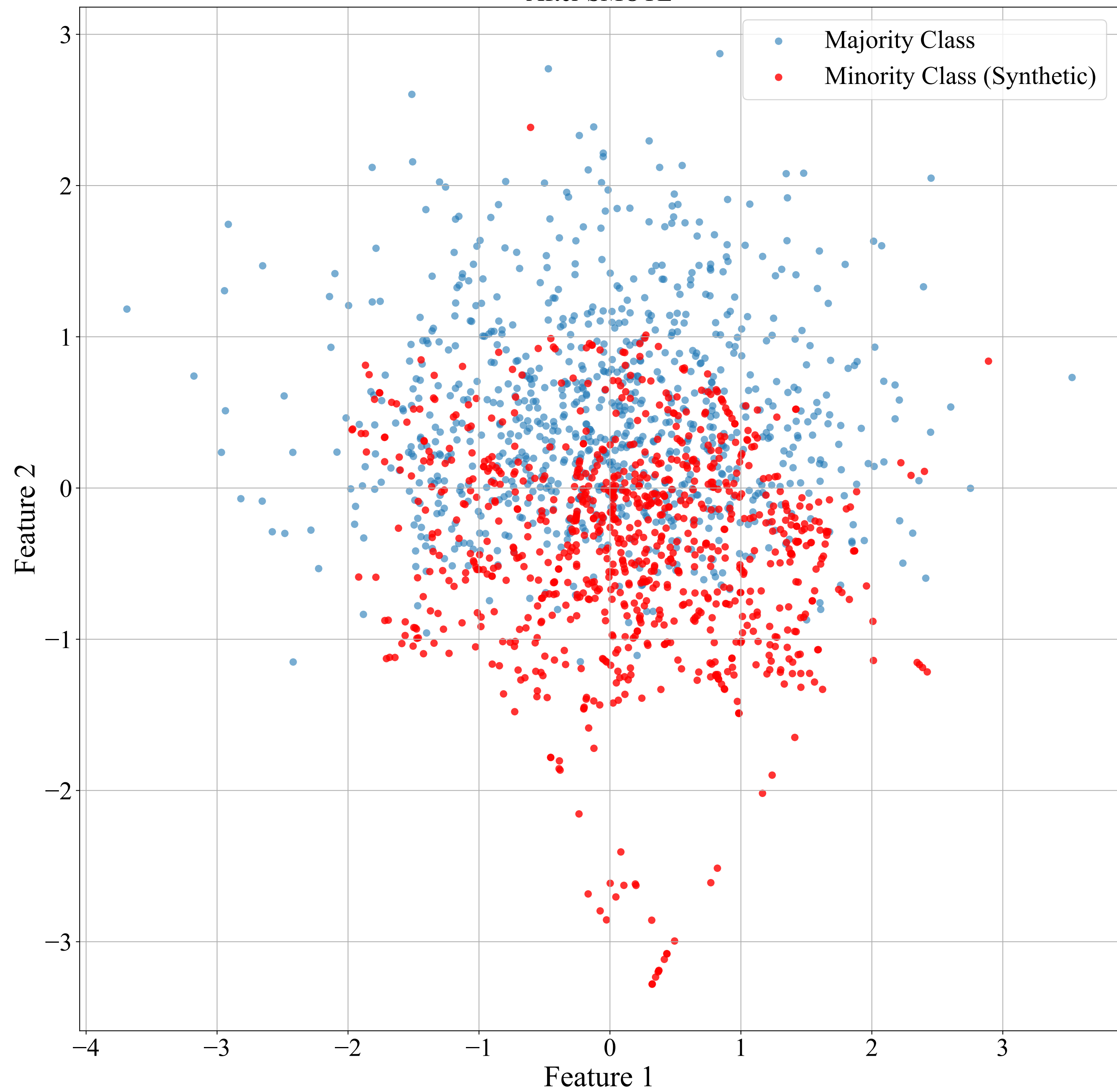
After SMOTE
