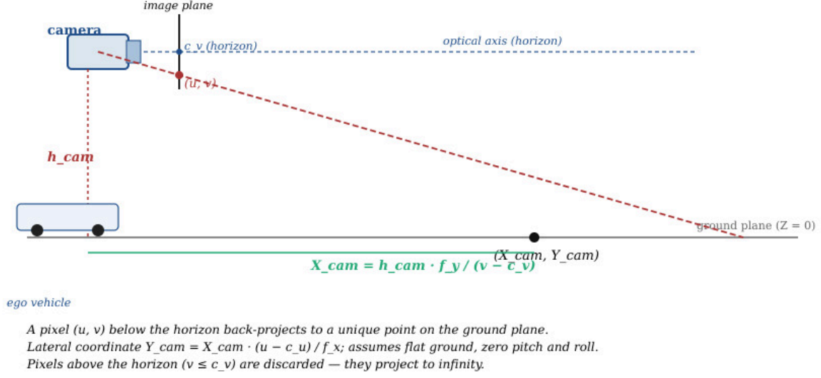
Figure 3.7: Inverse perspective mapping (side view). A pixel below the horizon back-projects to a unique point on the ground plane, given the camera height h_{cam} and the camera intrinsics (f_x, f_y, c_u, c_v) . Pixels above the horizon v \leq c_v project to infinity and are discarded.
