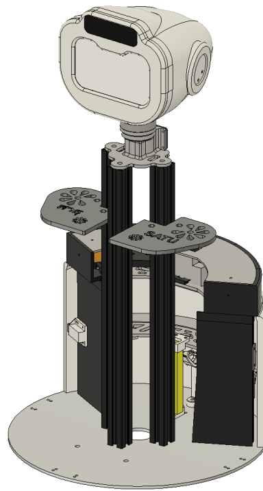
Figure 3.5 Upper Body Interior Structure
