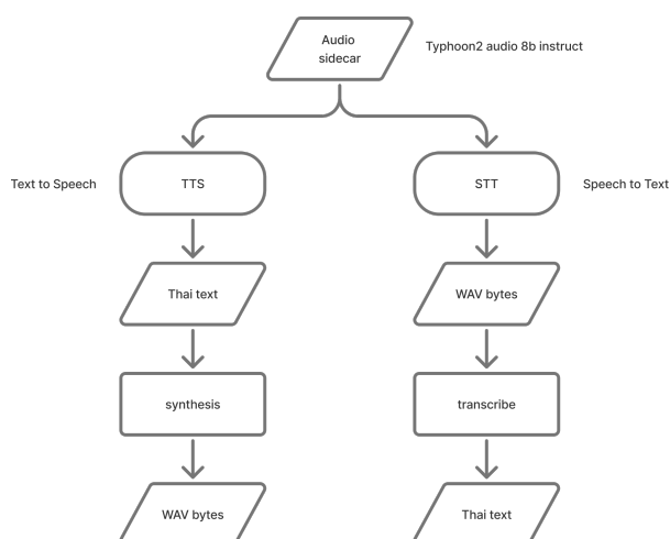
Figure 3.19 Audio Sidecar Service: TTS Synthesis and STT Transcription Processing Flows (Port 8001)
