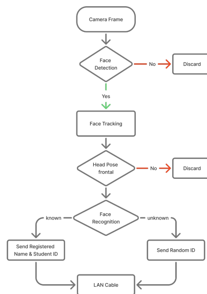
Figure 3.21 JetsonVision Pipeline: Face Detection, Multi-Object Tracking, Head Pose Gating, and Recognition
