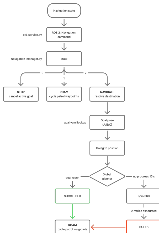
Figure 3.26 Autonomous Navigation State Machine: Goal Dispatch, Stuck Detection (360° Recovery), and Retry Logic
