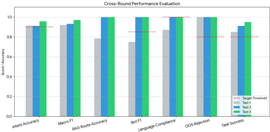
Figure 4.3 Cross-Round Performance Evaluation
