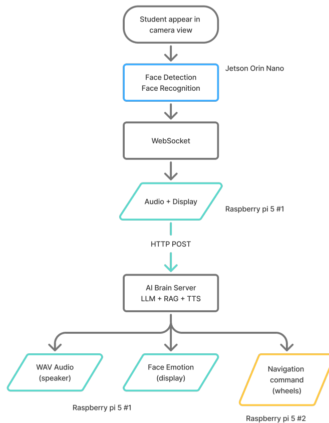
Figure 3.1 System Overview: Distributed Node Architecture and Communication Pathways
