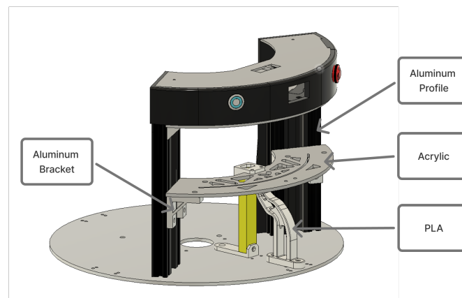
Figure 3.7 Material in Battery Tray Design
