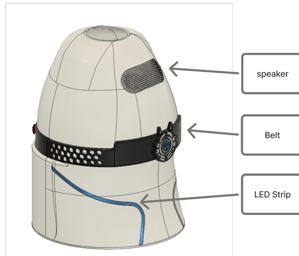
Figure 3.4 Upper Body Design
