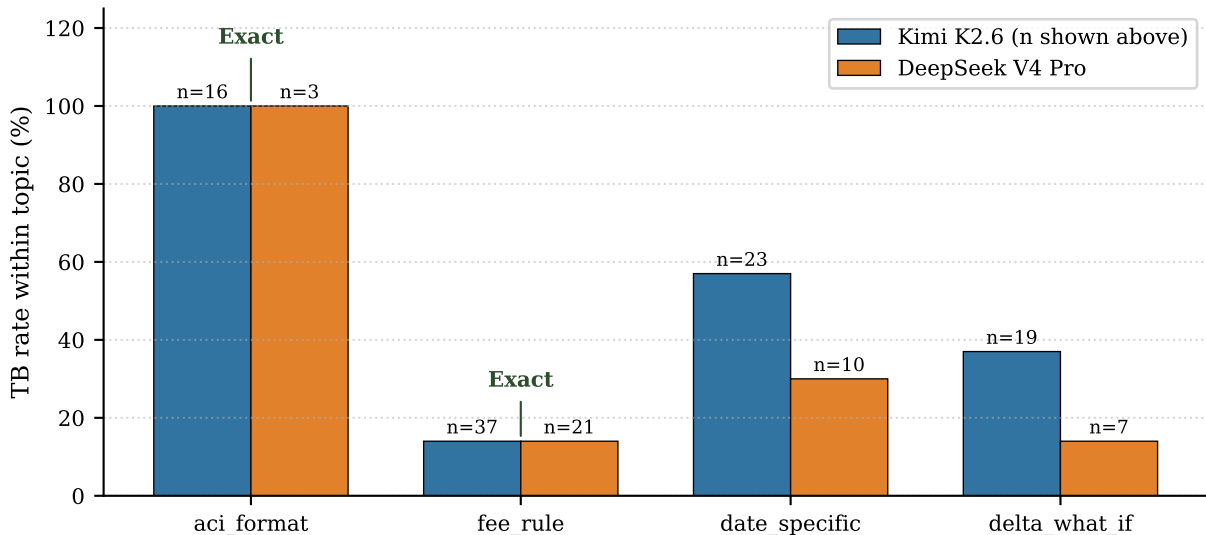
Per-topic TB rate replicates exactly on the two dominant clusters
