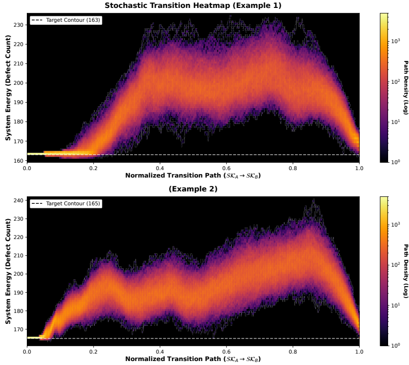
Figure 8: A logarithmic path density heatmap mapping 1000 stochastic transition walks between a single \mathcal{SK} pair (each example uses a separate pair). The fragmentation of these near-optimal SFPGS paths highlights the lack of continuous isentropic manifolds.
