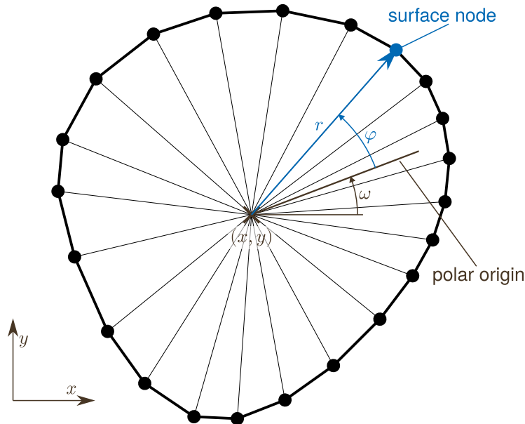
Figure 5.1: Position of a Particle and Its Local Coordinate System
