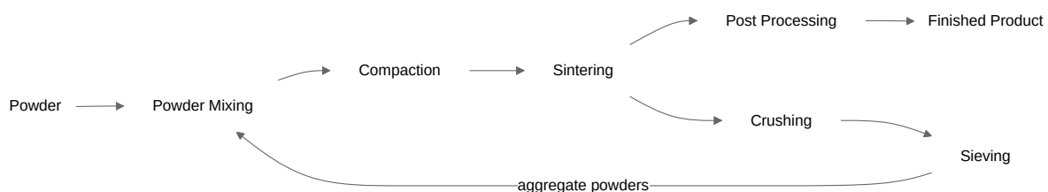
Figure 1.1: Chart of Common Process Steps for Sintered Products
