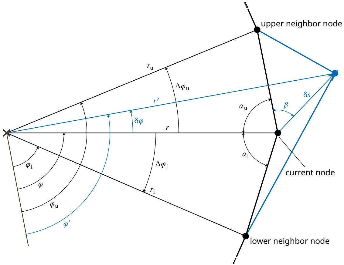
Figure 5.3: Geometry Overview of a Node Element
