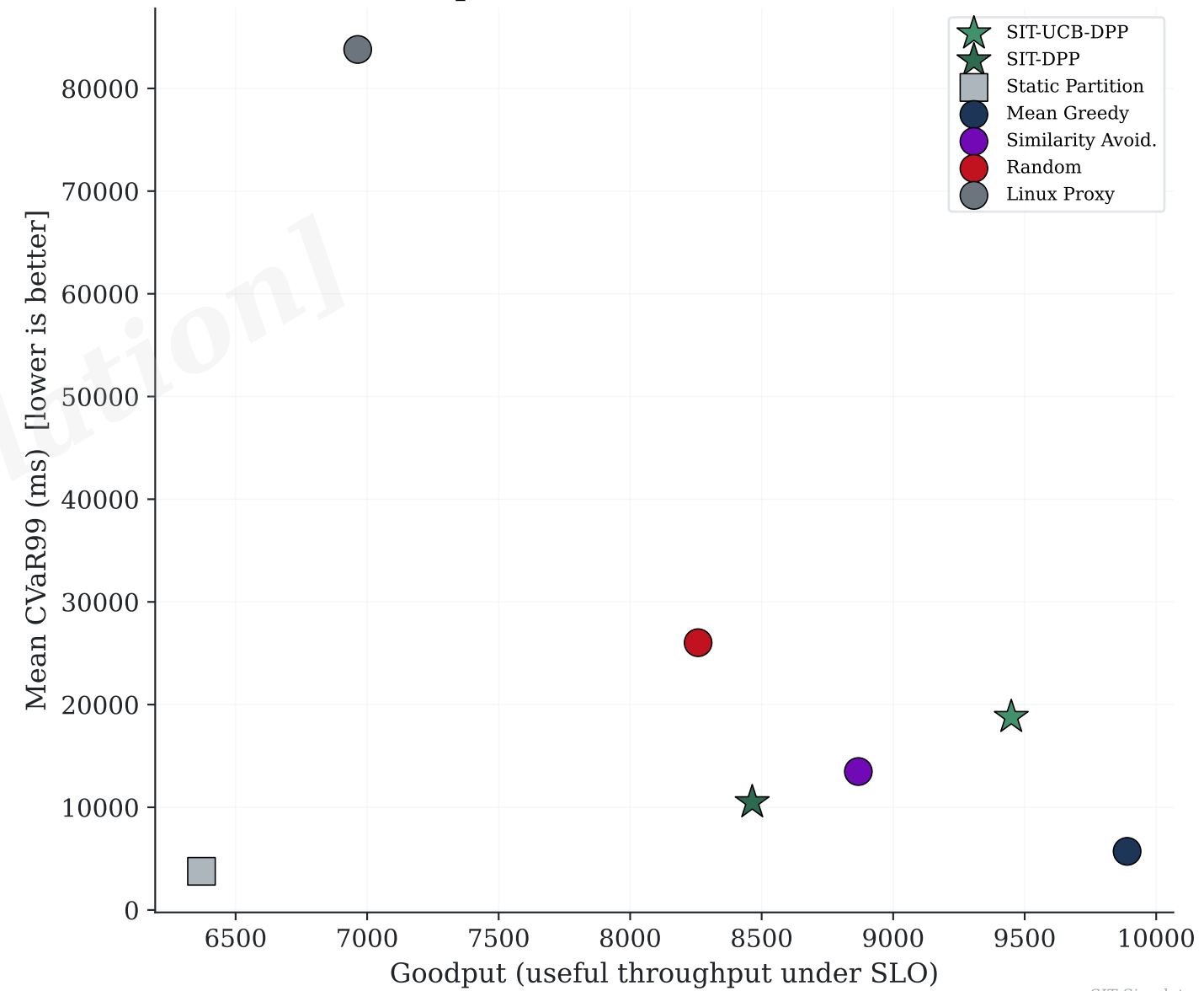
B. Goodput vs CVaR99 — SIT Dominates
