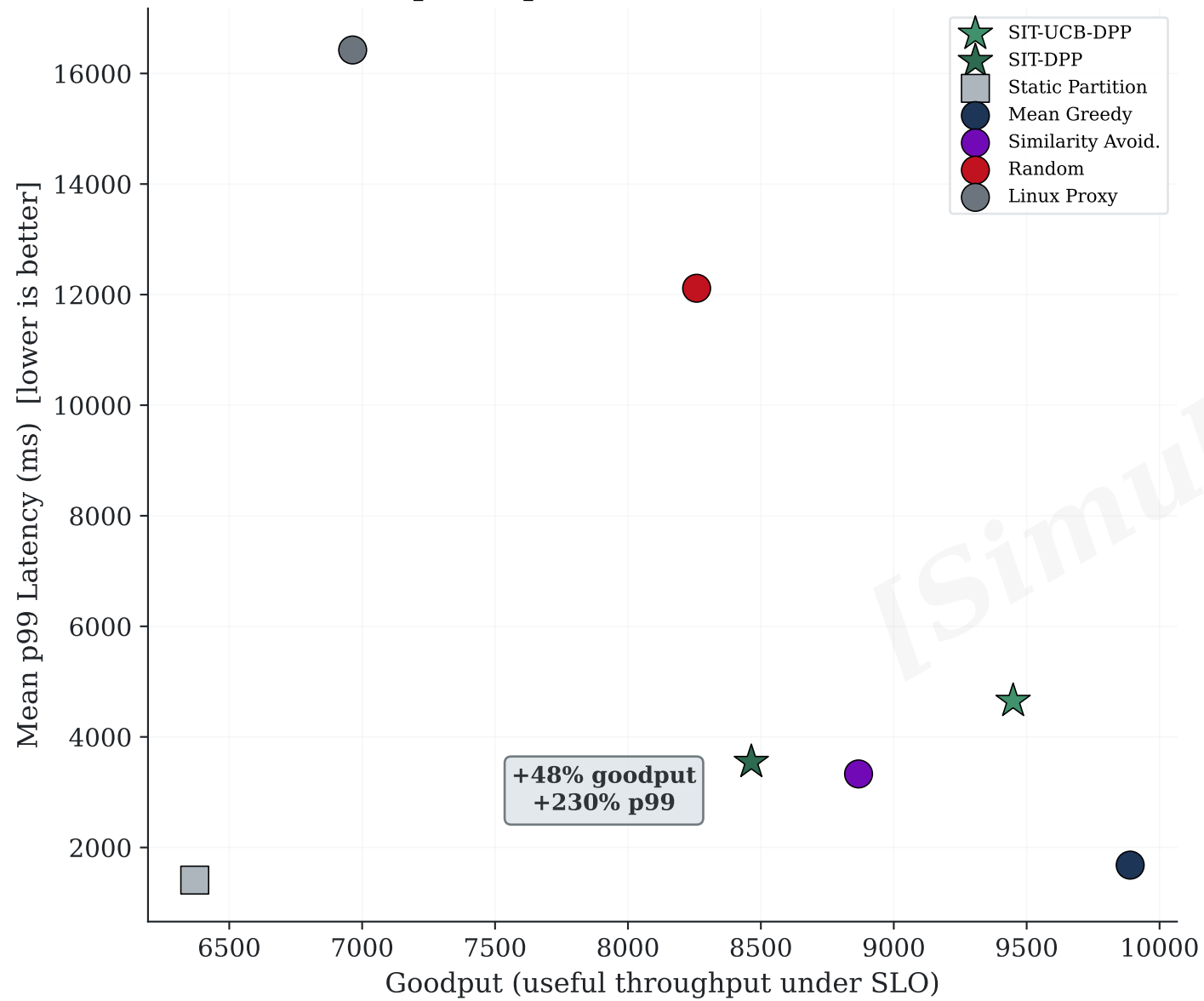
A. Goodput vs p99 — The Partition Trade-Off
