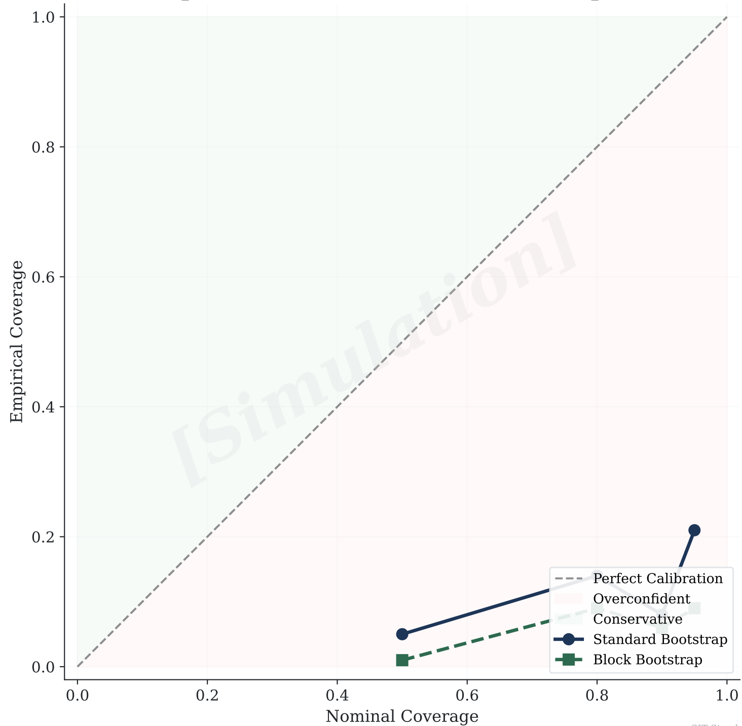
F19: Bootstrap CI Calibration -- Nominal vs Empirical Coverage
