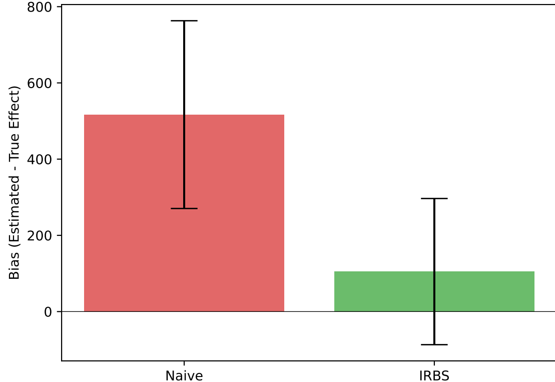
Measurement Bias Comparison
