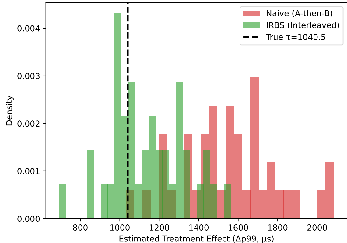
Distribution of Effect Estimates Under Drift
