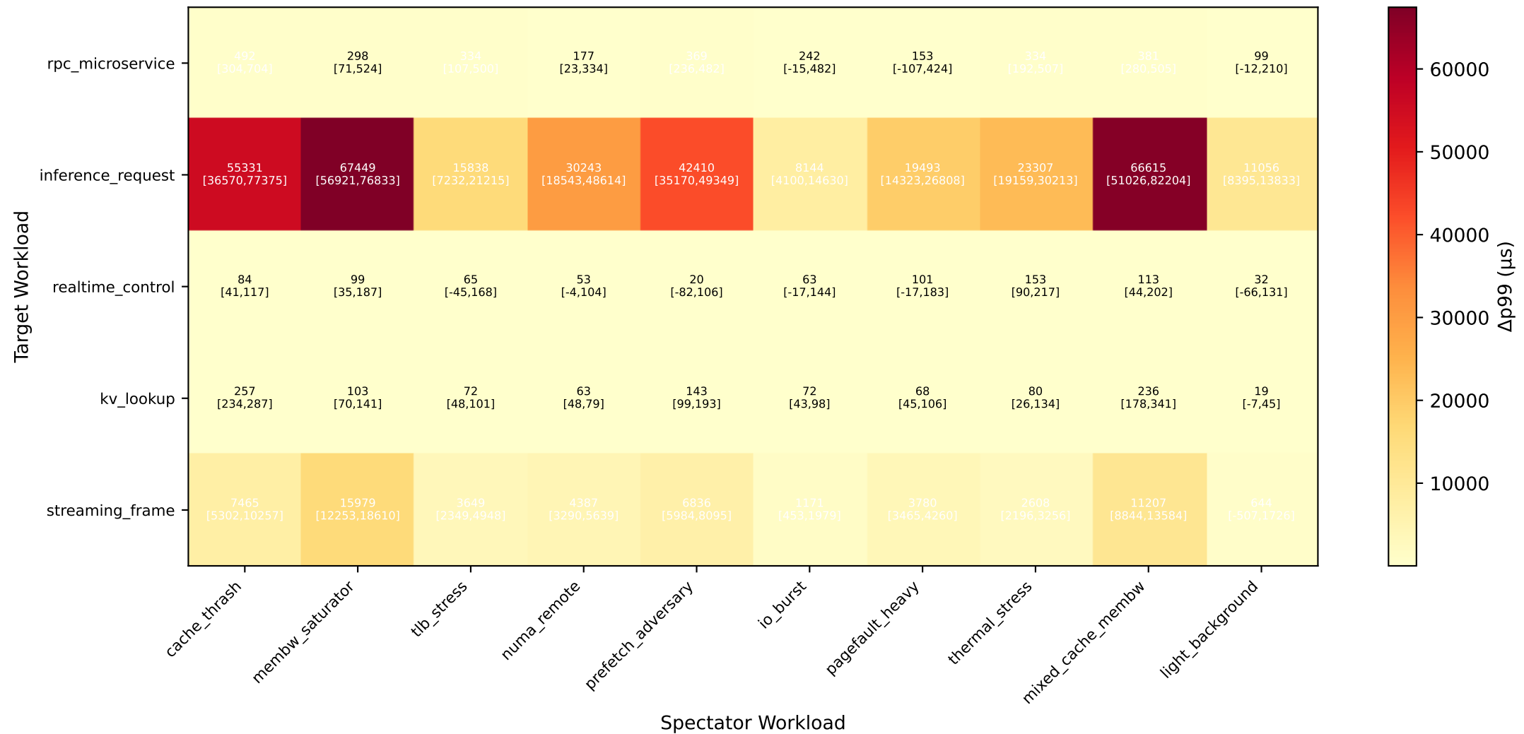
F3: Interference Tomography Map with Uncertainty [Simulation]
