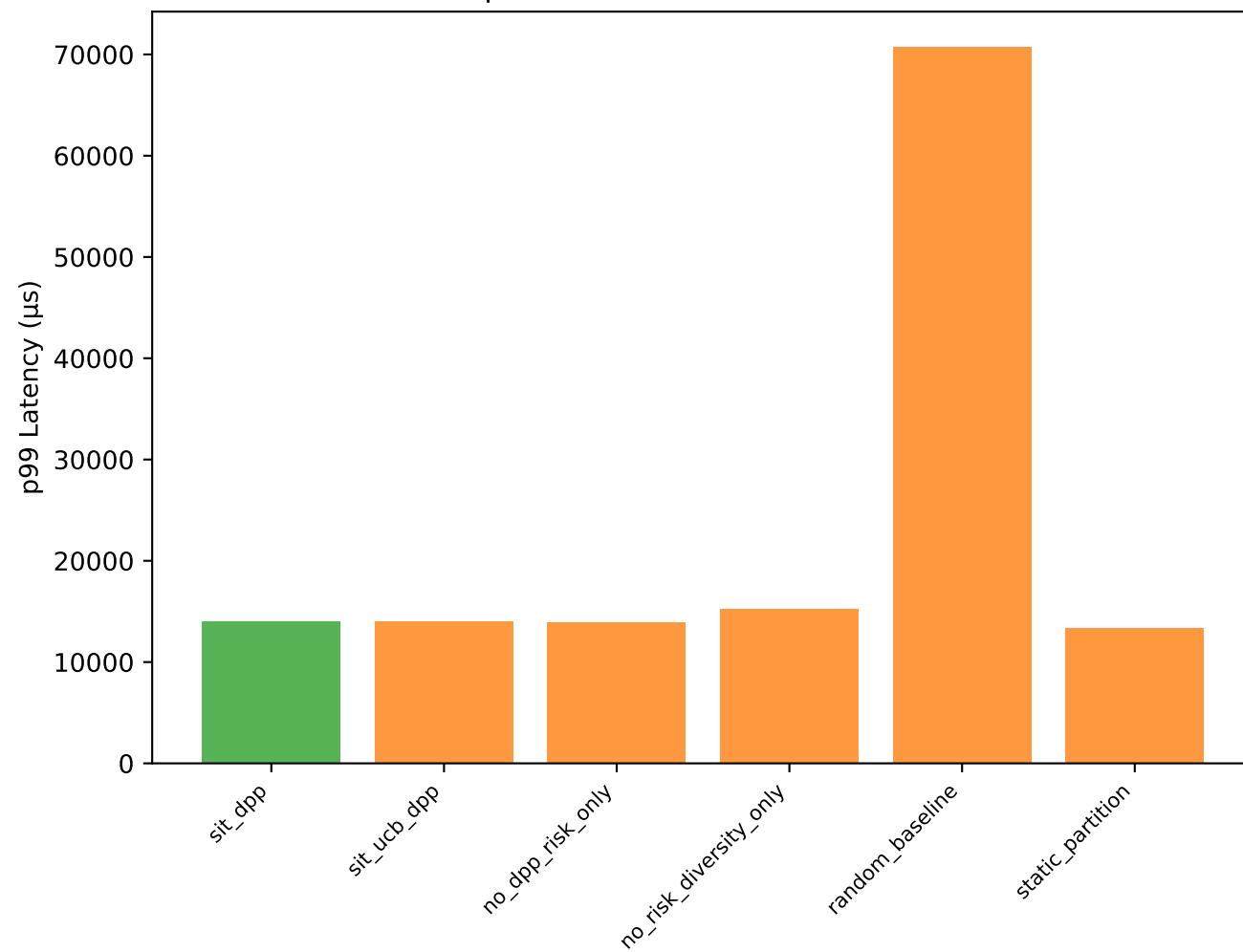
p99 Across Ablation Variants
