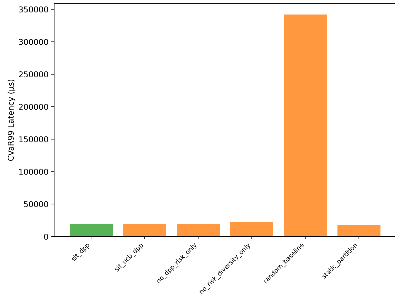
CVaR99 Across Ablation Variants
