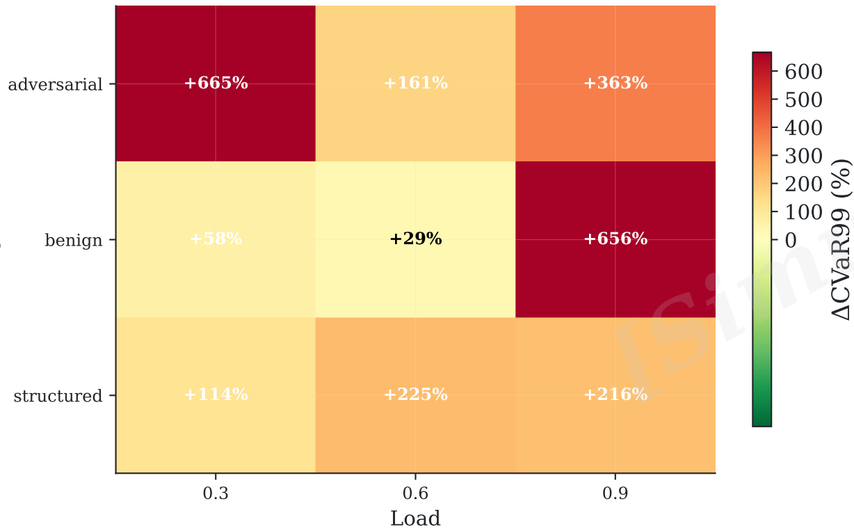
A. \Delta\text{CVaR99} (%) vs Best Non-SIT by Regime \times Load
