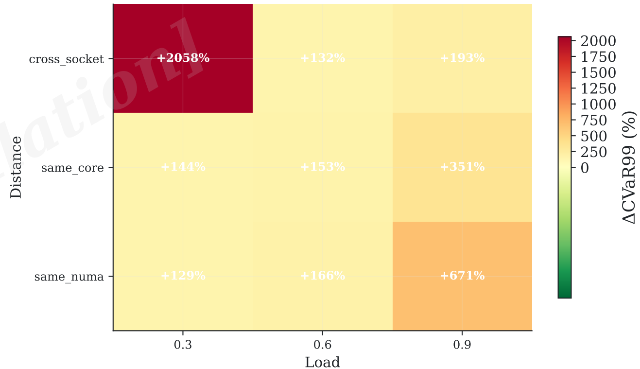
B. \Delta\text{CVaR99} (%) vs Best Non-SIT by Distance \times Load
