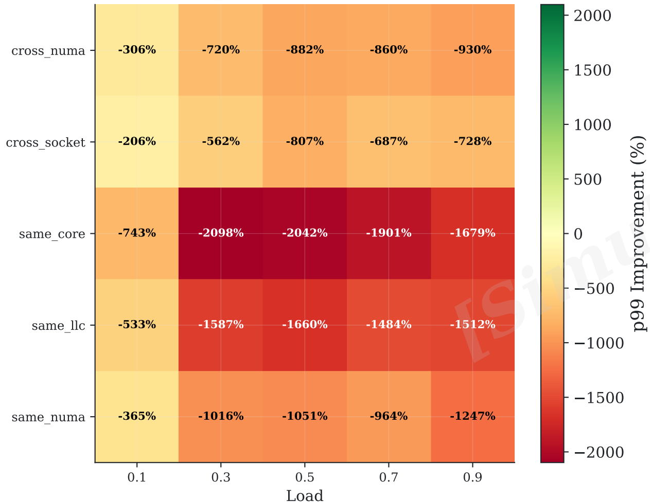
A. SIT p99 vs Best Baseline (%)
