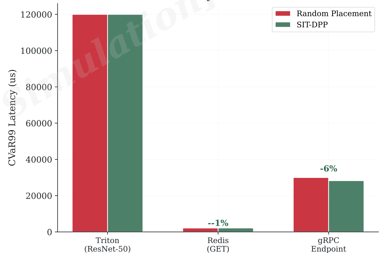
B. CVaR99 Latency: Random vs SIT-DPP
