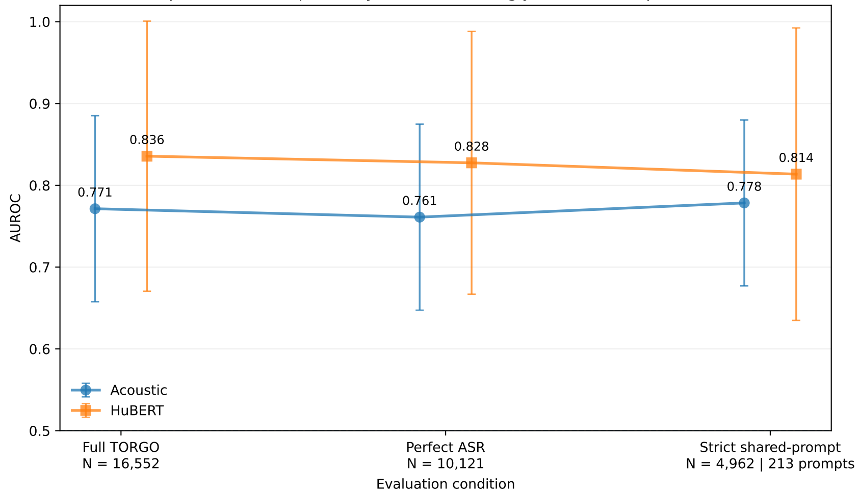
Speech-status separability under increasingly strict transcript controls
