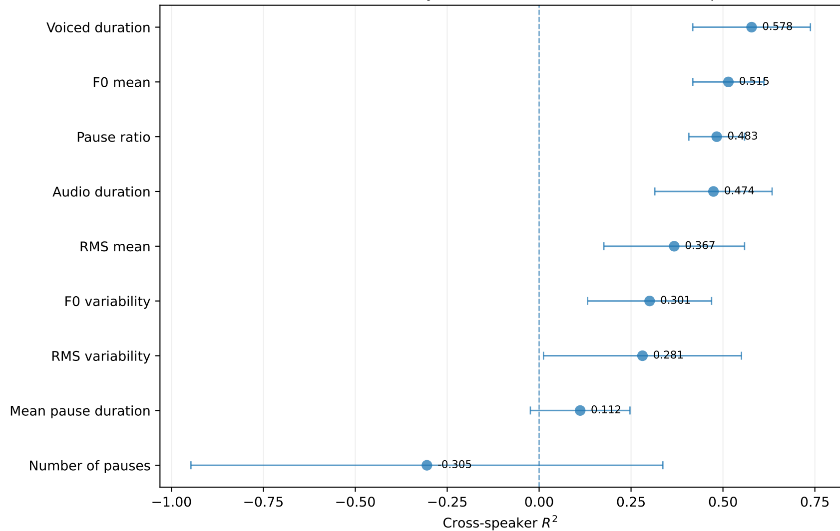
Acoustic characteristics linearly accessible from frozen HuBERT representations
