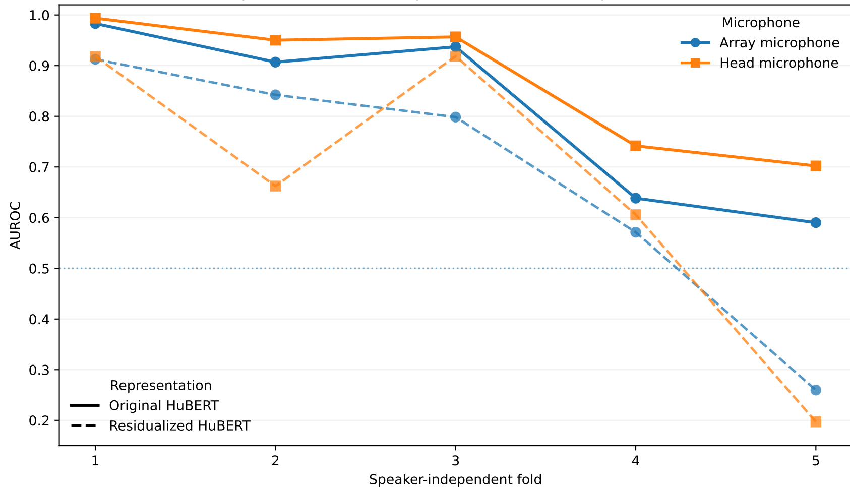
HuBERT performance across speaker folds and microphone conditions
