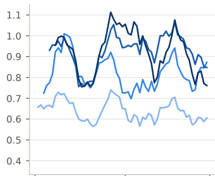
Spread / RMSE
