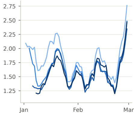
NeuralGCM
